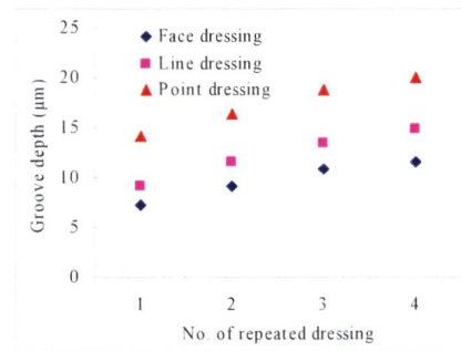
Fig. 11 Variation of groove depth for repeated dressing
