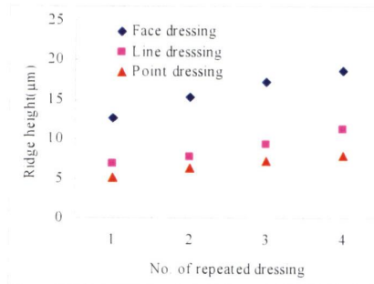
Fig. 12 Variation of ridge height for repeated dressing
