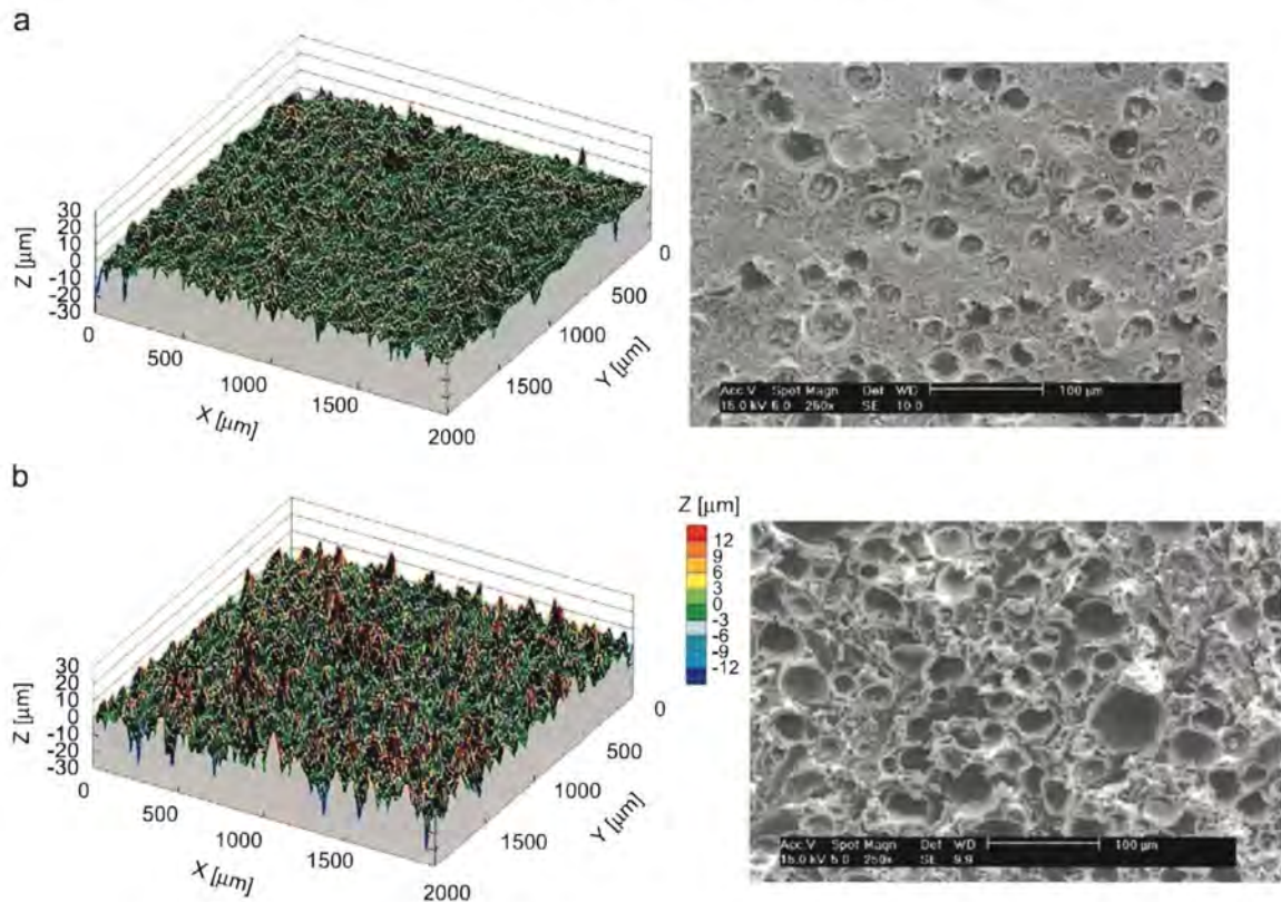
Fig. 4. The images of the pad surface formed by (a) ADD and (b) CDD.
