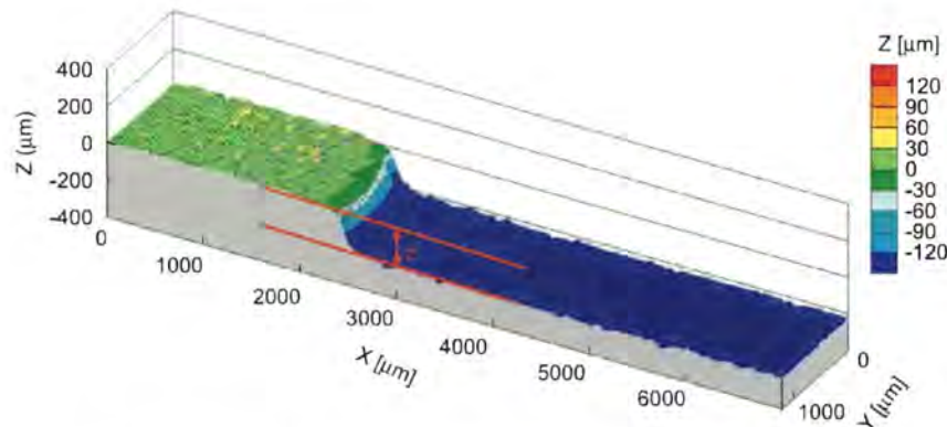
Fig. 9. 3D image of pad surface after 60 min dressing and Z is the pad thickness removed.
