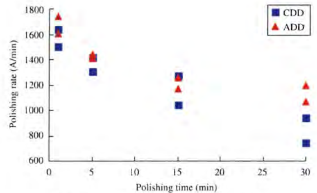
Fig. 12. Variation in polishing rate with polishing time.
