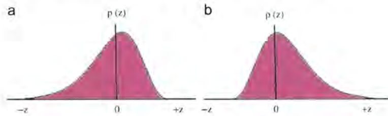
Fig. 6. Schematic drawing of the notion of skewness; (a) negative skewness and (b) positive skewness.
