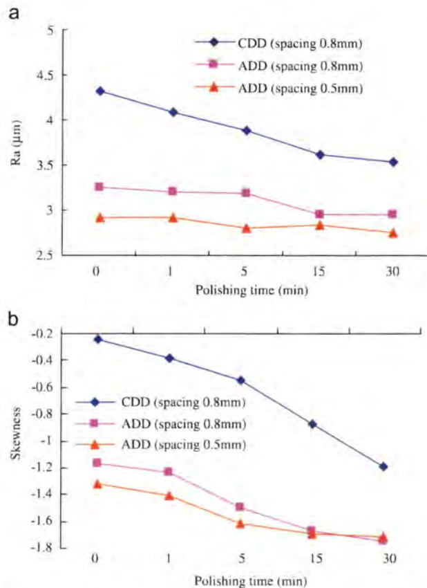
Fig. 11. Variation in surface roughness R_a (a) and skewness (b) with polishing time.
