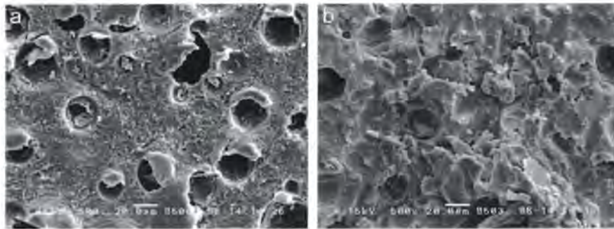
Fig. 13. SEM images of pad surface formed by (a) ADD and (b) CDD without conditioning of 30 min.
