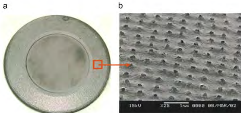
Fig. 2. (a) Conventional diamond dresser (CDD) and (b) an SEM micrograph of diamond grits attached to a flat substrate by brazing to form cutting tips.
