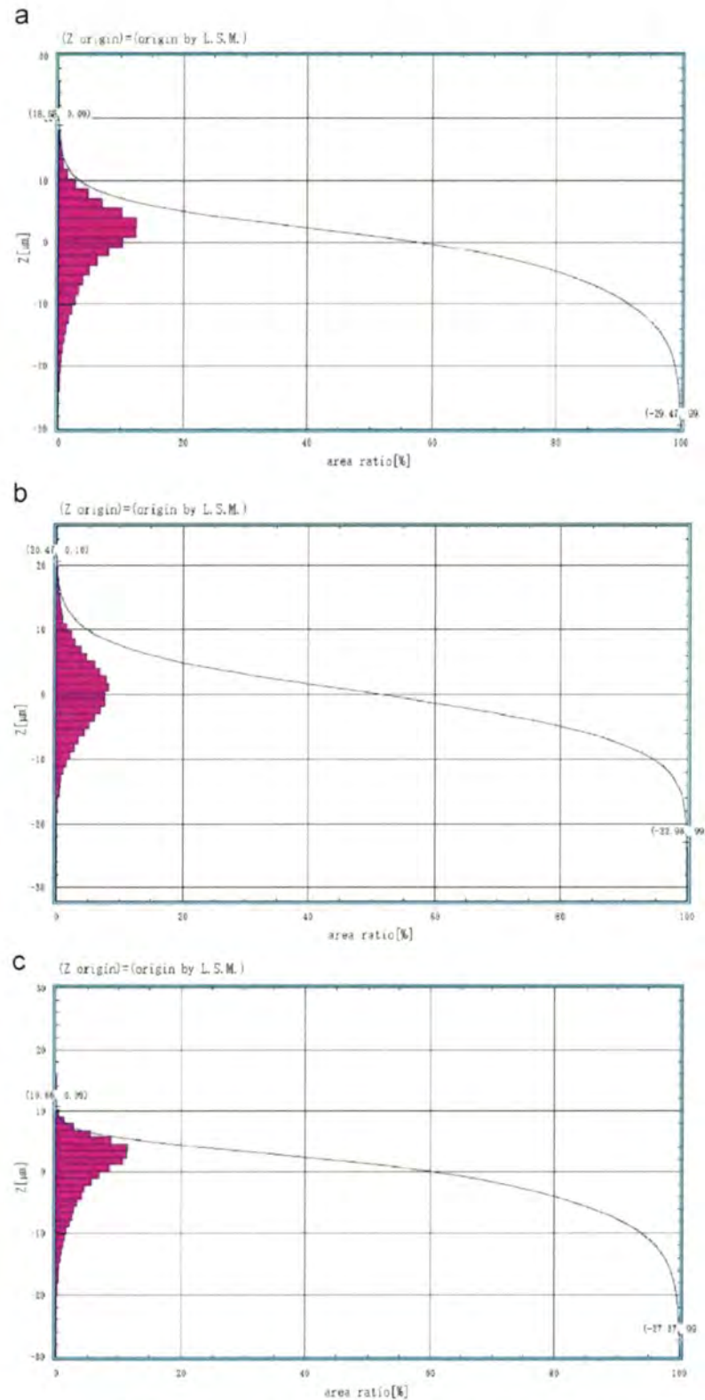
Fig. 7. Representative height probability distributions of the pad surface: (a) unused pad (b) CDD and (c) ADD after 60 min of dressing.
