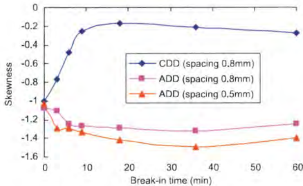
Fig. 8. Variation in skewness with break-in time.
