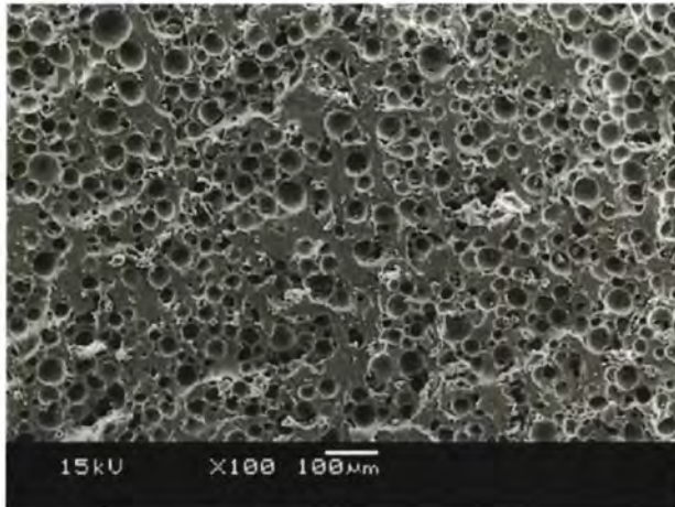
Fig. 1. SEM images of unused pad surface (IC1000).
