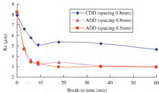
Fig. 5. Variation of surface roughness R_a with break-in time.
