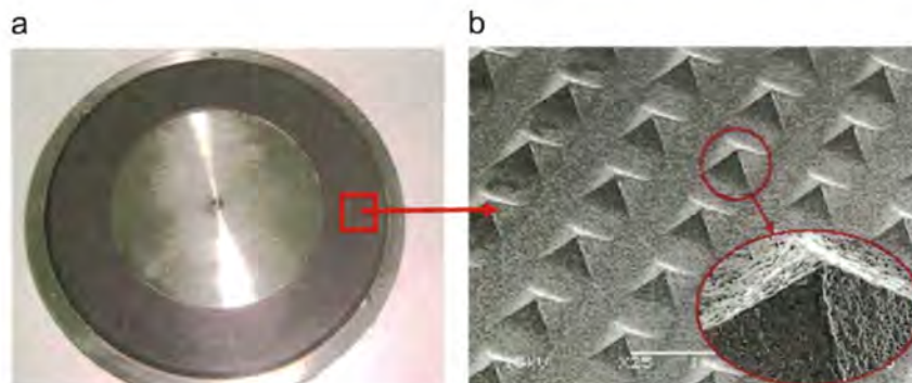
Fig. 3. (a) Advanced diamond dresser (ADD) and (b) an SEM image of cutting pyramids formed on the surface of a polycrystalline diamond.
