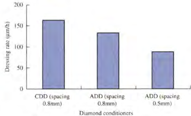
Fig. 10. Variation in dressing rate with diamond conditioners.
