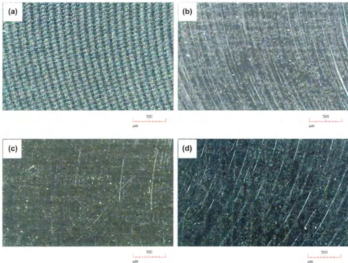
Figure 9. Cross-sectional SEM images of workpiece surface with (a) dry; (b) MQL; (c) CSMQL; and (d) wet machining.
