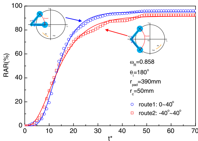
Fig. 14 The influence dressing routes on the resulted RAR
