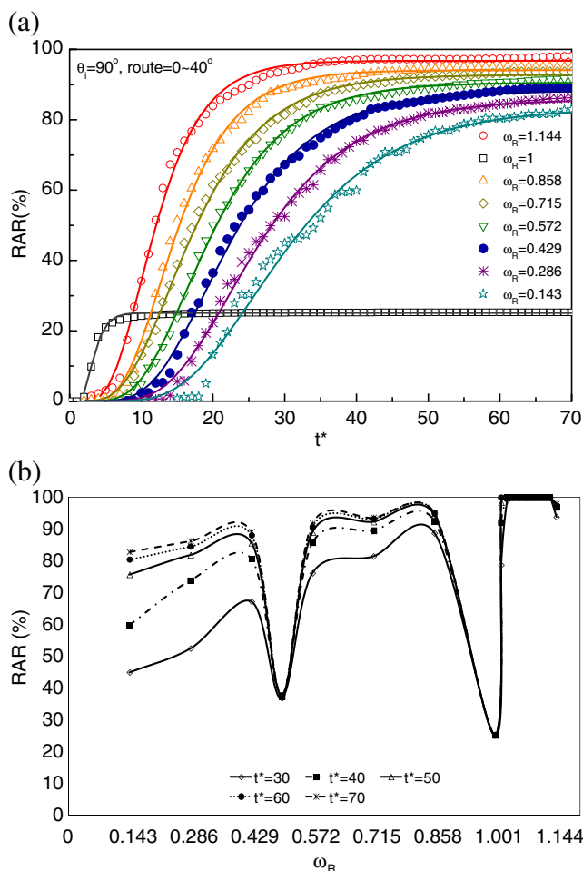
Fig. 12 The influence of \omega_R on the resulted RAR, a the time histories with different \omega_R , b the resulted RAR of various \omega_R at different t^*
