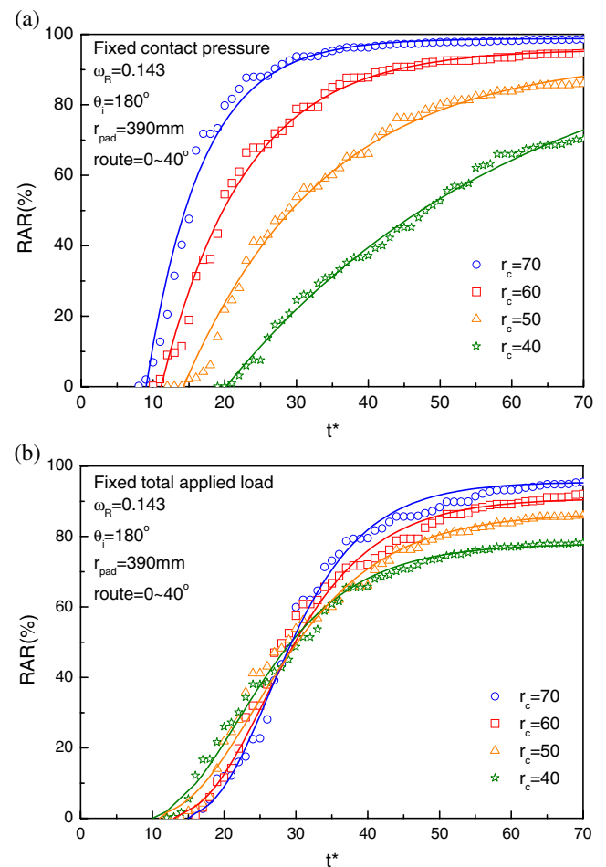
Fig. 15 The influence of dresser disk size on the resulted RAR, a the back pressure is fixed, b the total back load is fixed
