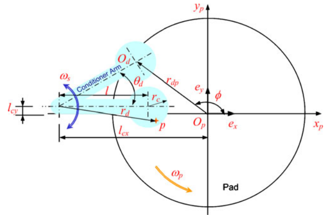
Fig. 2 The schematic of pad/dresser system and the definitions of necessary parameters
