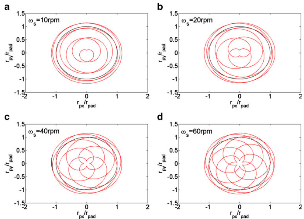
Fig. 6 Trajectories on the pad generated by one grain on the dresser center with different rotating speed \omega_s . a \omega_s=10 rpm, b \omega_s=20 rpm, c \omega_s=40 rpm, d \omega_s=60 rpm (horizontal axis: r_{px}/r_{pad} , vertical axis: r_{py}/r_{pad} )
