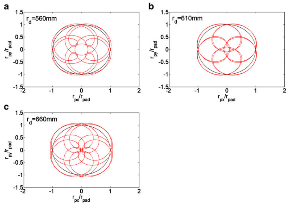
Fig. 8 Trajectories on the pad generated by one grain on the dresser with different r_d , a r_d=560 mm, b r_d=610 mm, c r_d=660 mm (horizontal axis: r_{px}/r_{pad} , vertical axis: r_{py}/r_{pad} )
