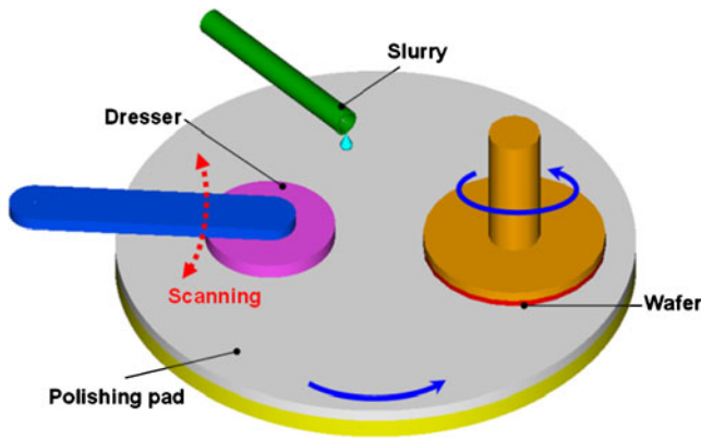
Fig. 1 Schematics of a CMP dresser system
