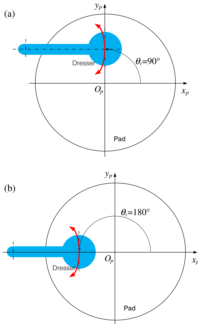
Fig. 4 Definitions of the dresser initial position, a \theta_i = 90^\circ , b \theta_i = 180^\circ
