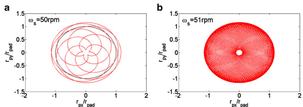
Fig. 7 Trajectories on the pad with different rotation ratio a \omega_s=50 rpm, b \omega_s=51 rpm (horizontal axis: r_{px}/r_{pad} , vertical axis: r_{py}/r_{pad} )
