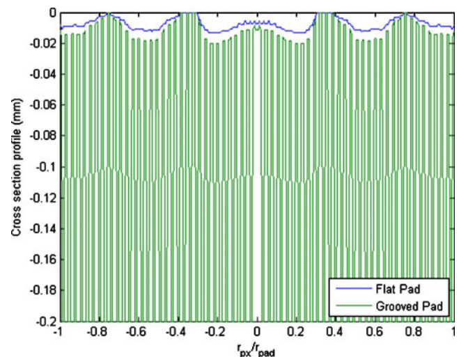
Fig. 11 The profile of ungrooved and grooved pads after t^* exceeds 70
