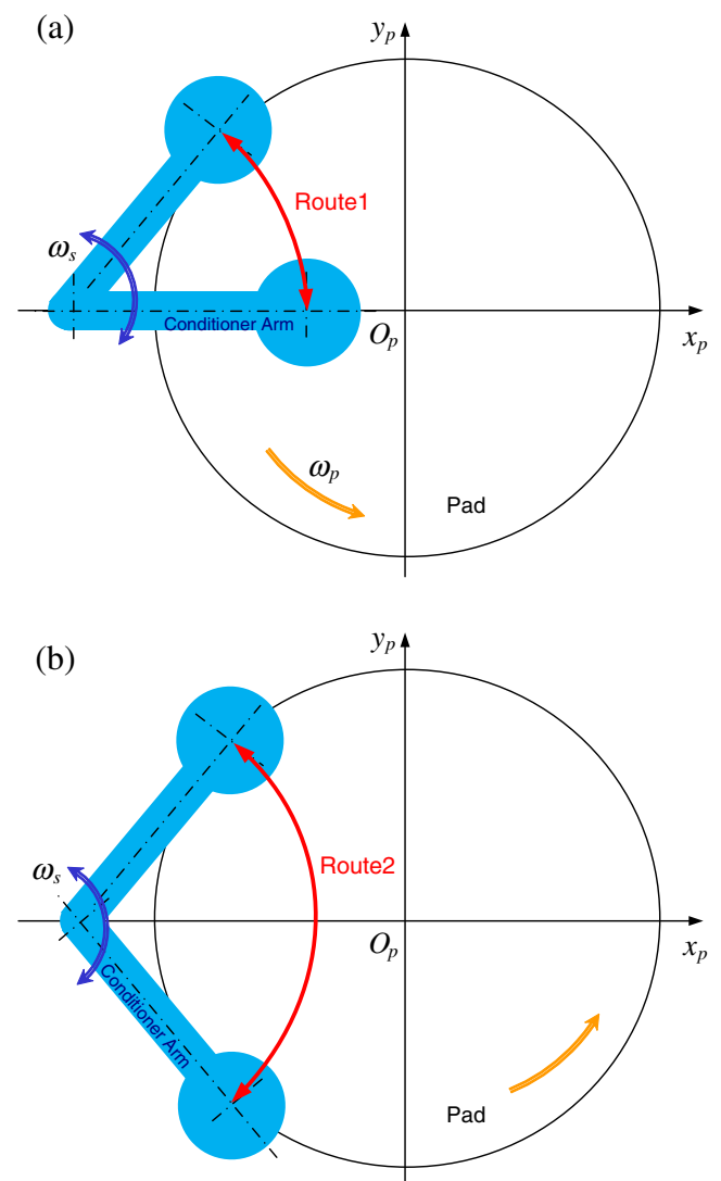
Fig. 5 Definitions of the dresser swing routes, a Route1 = 0 \sim \theta_s , b Route2 = -\theta_s \sim \theta_s
