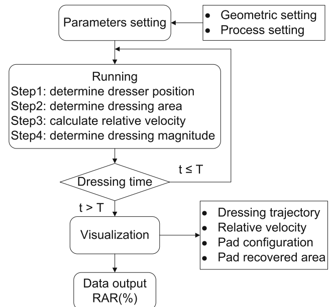
Fig. 3 Schematic of pad conditioning simulation module
