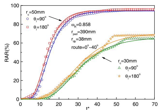
Fig. 13 The influence of the dresser initial position on the achieved RAR
