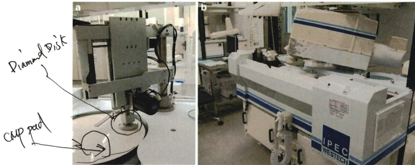
Fig. 4 a Dressing system and b polishing system
