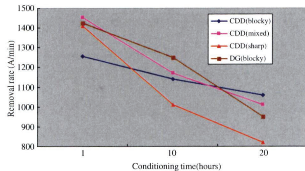
Fig. 12 Variation in wafer removal rate dressed by CDD and DG
