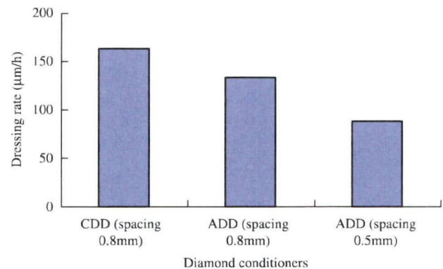
Fig. 10. Variation in dressing rate with diamond conditioners.
