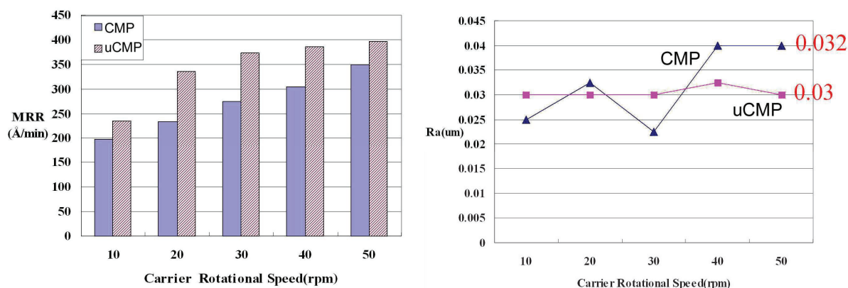
Fig. 12: The increased wafer removal rate at different wafer rotational speed by inducing ultrasound during CMP.
