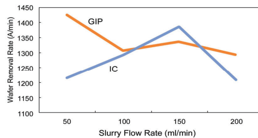
Fig. 7: The oxide removal rate as a function of slurry flow rate. Note that at 50 ml/min, GiP can polish wafer faster than IC even the latter was with 3X of slurry consumption.
