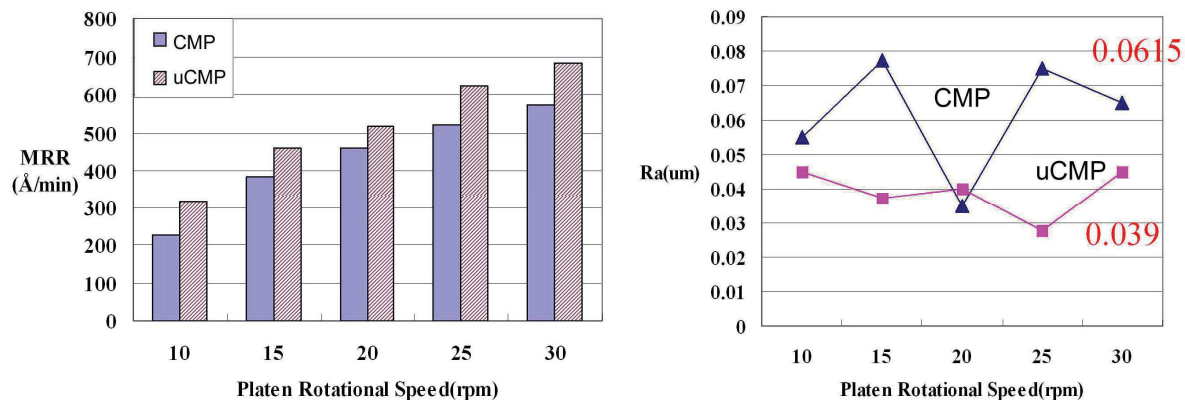
Fig. 11: The increase of wafer removal rate and the decrease of wafer surface roughness can be both achieved by implementing ultrasound CMP (uCMP) at a wide range of platen's rotational speed.
