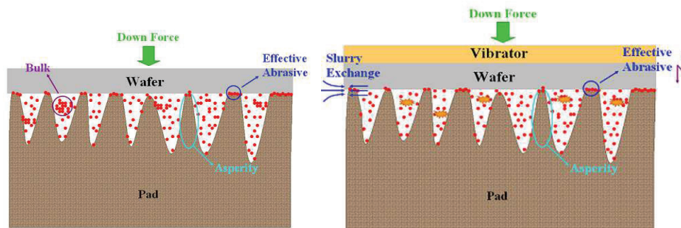
Fig. 10: The illustration of ultrasonic effects on the dispersion of slurry in the asperities of pad surface.
