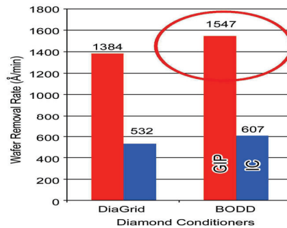
Fig. 6: The dramatic increase of polishing rate during oxide CMP by using the black GiP pad compared to conventional white IC pad. The advantage of using GiP is further enhanced by using BODD as the diamond dresser.
