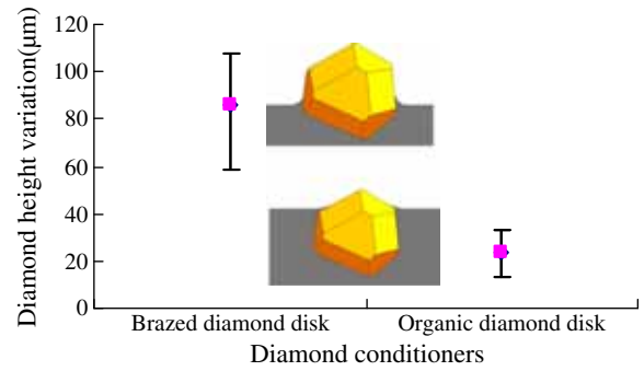
Fig. 6. Height variation in tips for diamond conditioners.
