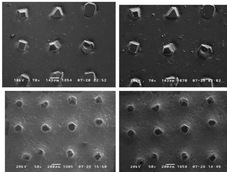
Fig. 8. SEM observation of the surface topography of the BDD after (a) 1 h and (b) 40 h and that of the surface topography of the ODD after (c) 1 h and (d) 40 h in the oxide-slurry solution.
