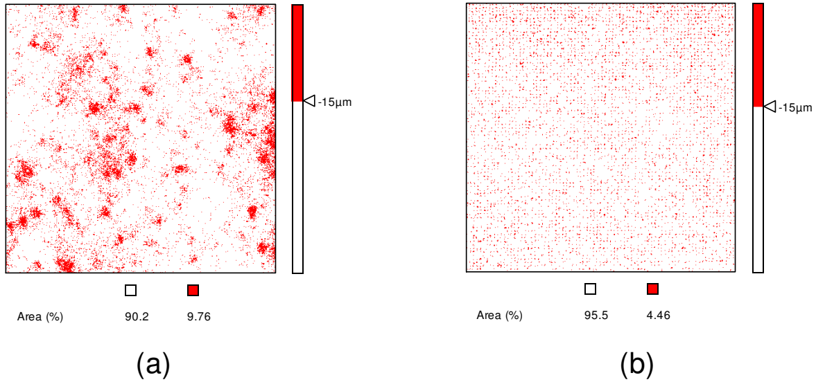
Figure 3. Surface topography slice at 15 μm elevation showing estimated contact area of the a) current and b) improved fine-finish disk designs.
