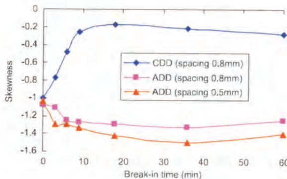
Fig. 8. Variation in skewness with break-in time.
