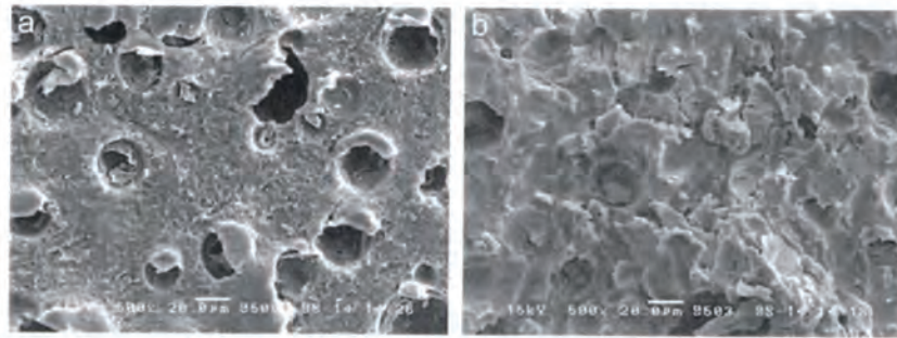
Fig. 13. SEM images of pad surface formed by (a) ADD and (b) CDD without conditioning of 30 min.
