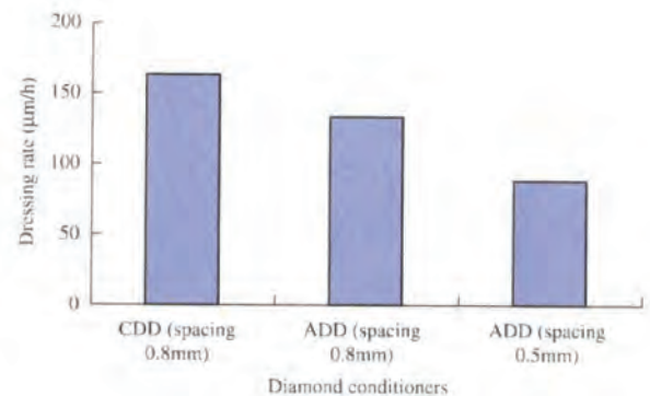
Fig. 10. Variation in dressing rate with diamond conditioners.
