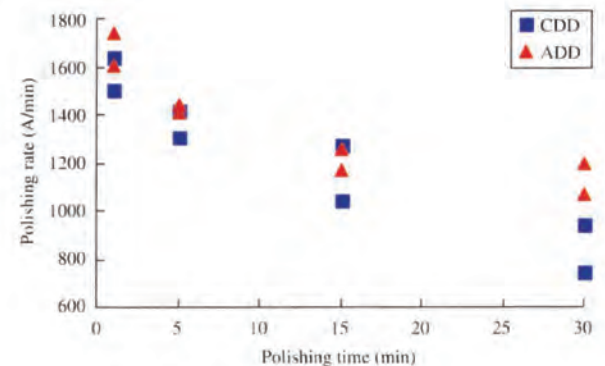
Fig. 12. Variation in polishing rate with polishing time.
