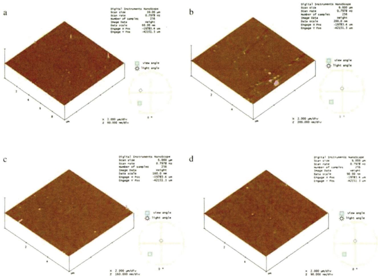
Fig. 9. AFM observation of polished surfaces of the BDD after (a) 1 h and (b) 40 h of dressing and that of the polished surfaces of the ODD after (c) 1 h and (d) 40 h of dressing.
