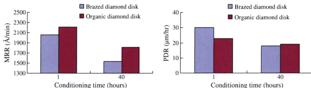
Fig. 7. Variation in the material removal rate of the wafer dressed by the brazed diamond disk and the organic diamond disk.
