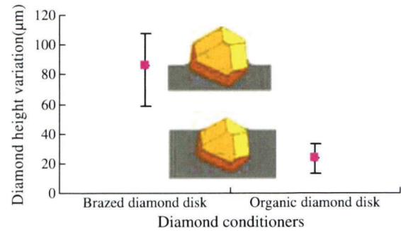
Fig. 6. Height variation in tips for diamond conditioners.
