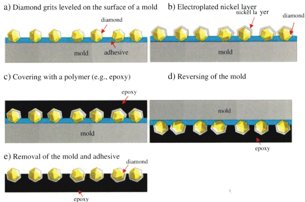
Fig. 2. Steps for manufacturing organic diamond disk.
