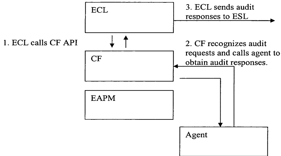
Figure 7b: Client Responding to Audit Requests
