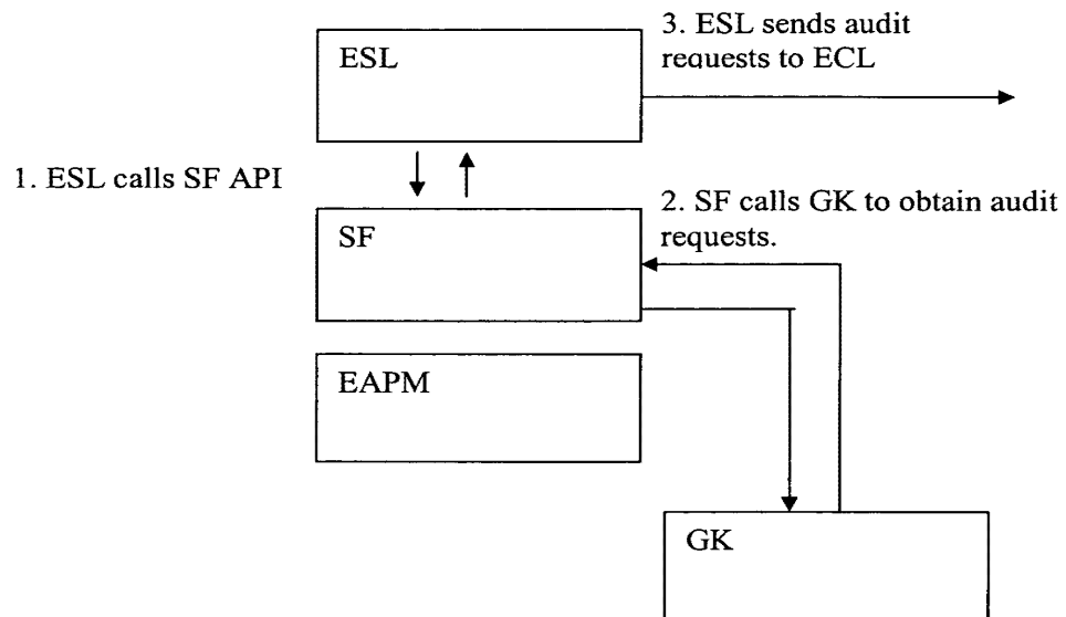
Figure 7a: Server in Audit State
