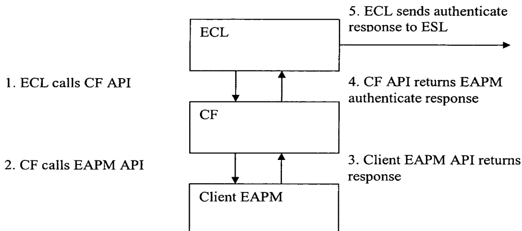
Figure 5a: Client in Authentication State
