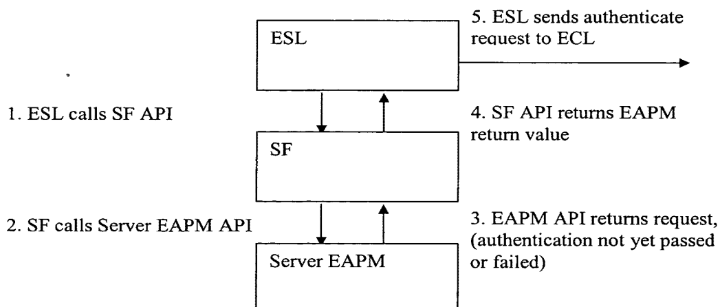
Figure 5b: Server in Authentication State
