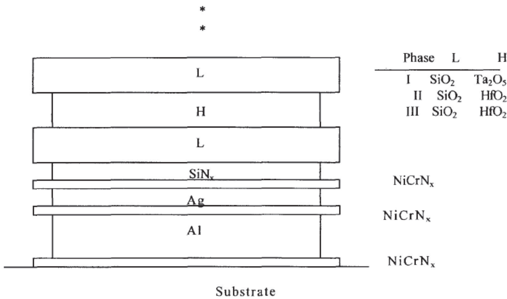
Fig. 2 Coating Design
