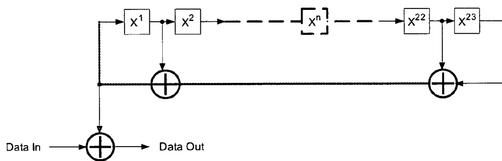
Data Scrambler with PN23
