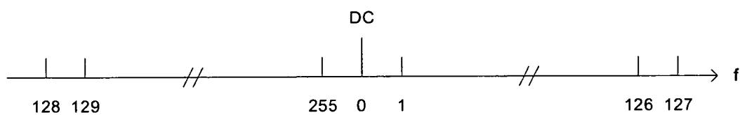
Figure 8 Sub-Carrier Numbering
