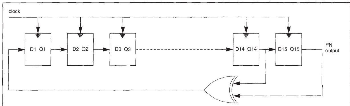
Fig. 7 A PN generator with polynomial 1 + x^{14} + x^{15}
