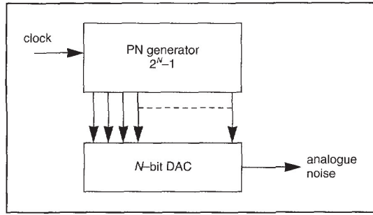
Fig. 6 An analogue noise source
