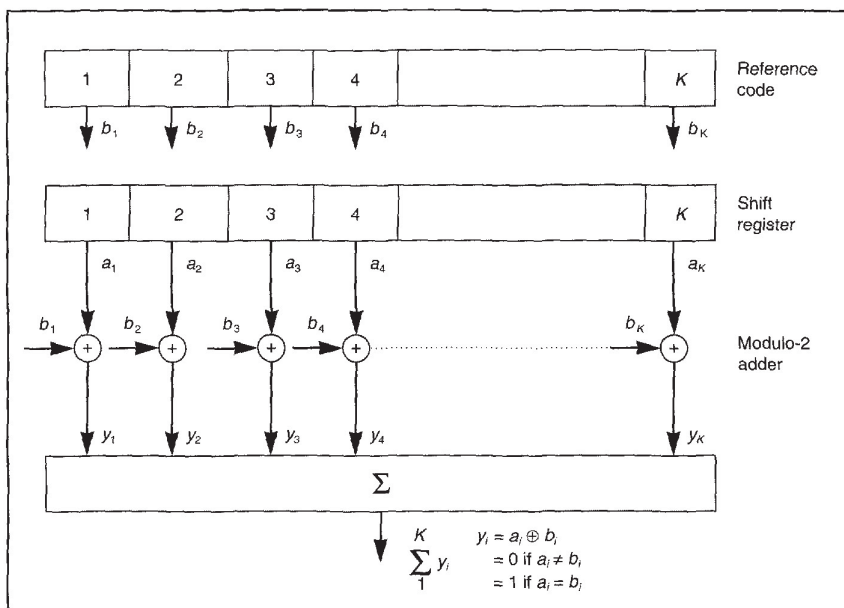
Fig. 2 A correlator
