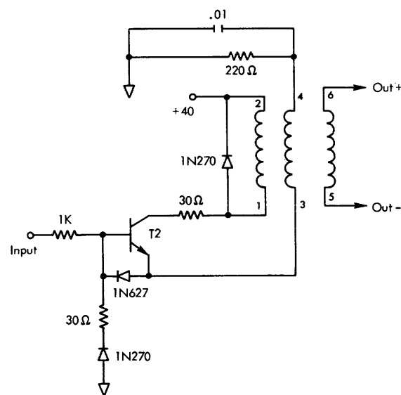
Figure 9. Blocking Oscillator.
