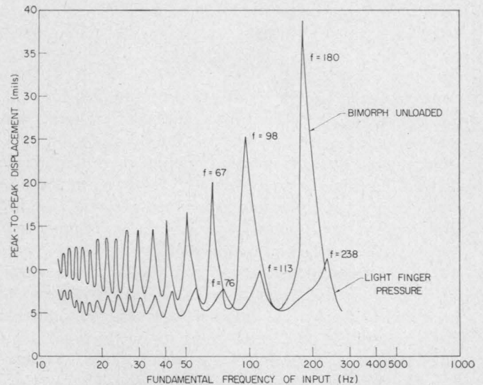
Fig. 5. Bimorph deflection as a function of the repetition rate of 2.6-ms driving pulses.
