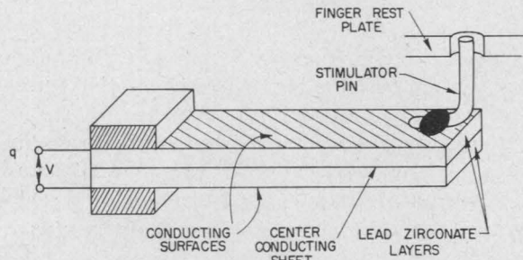
Fig. 3. Piezoelectric bimorph reed mounted for use as a tactile stimulator.
