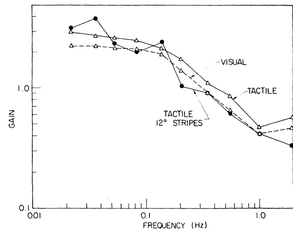
Fig. 13. Pursuit-tracking gain as a function of frequency with the environment sensor.
