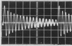
Fig. 6. Lightly loaded bimorph driven by rectangular pulses 2.6 ms in duration and 80 ms apart. Horizontal scale: 10 ms/div. Vertical scale: 2.5 mils/div.
