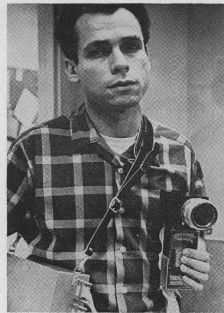
Fig. 11. Optical-to-tactile image-conversion unit for environment sensing. In the operator's left hand is the optical unit and the tactile stimulator array. Battery-operated electronics are carried under the right arm.
