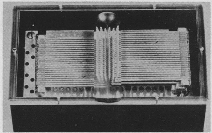
Fig. 7. Tactile stimulation array. The 24-by-6 array of tactile stimulators fits on one fingertip. The stimulator pins are spaced 50 mils apart along the finger and 90 mils apart across the finger. The perforated surface is curved to fit the finger.
