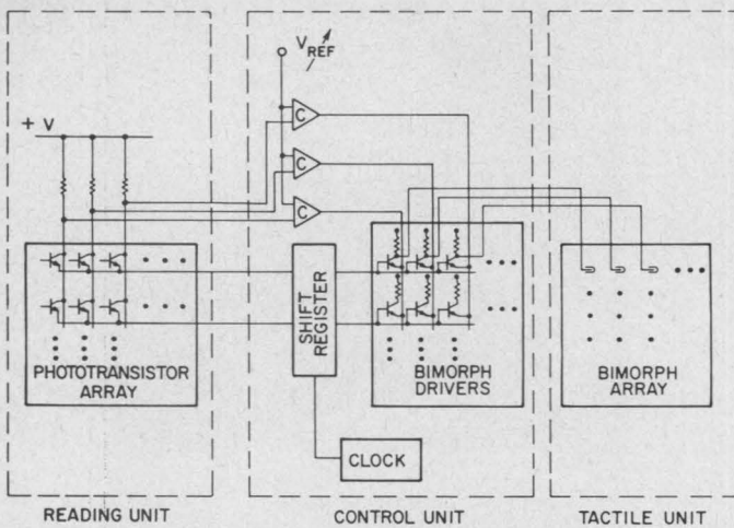
Fig. 2. Simplified block diagram of multiplex electronics. The shift register specifies which row of six bimorph drivers is to receive signals from the six phototransistors in the corresponding row. Thus, the phototransistor signals are transferred, one row at a time, to the bimorph drivers, over six wires.
