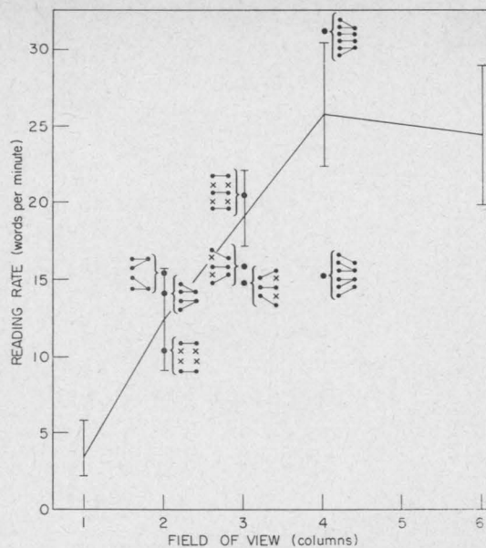
Fig. 10. Reading rate as a function of field of view and phototransistor-to-stimulator mappings. Line and vertical bars indicate results as the number of phototransistor columns is varied. Right-hand dots indicate phototransistor columns and left-hand dots indicate bimorph columns. Connecting lines indicate phototransistor-column to bimorph-column mappings.
