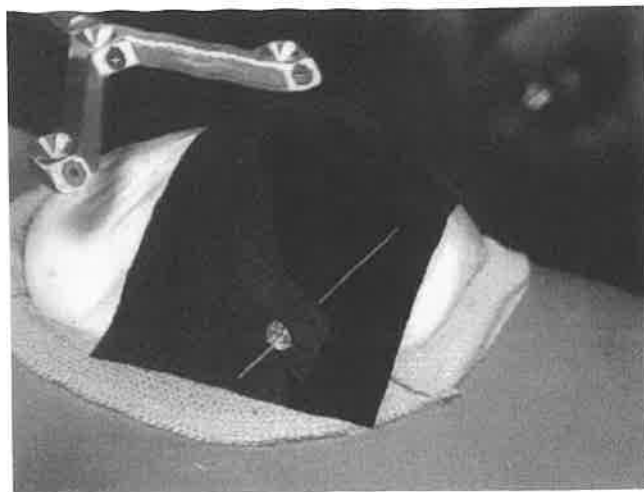
Figure 3. Mockup of breast tumor biopsy. 3D graphics guide needle insertion. (Courtesy Andrei State, UNC Chapel Hill Dept. of Computer Science.)
