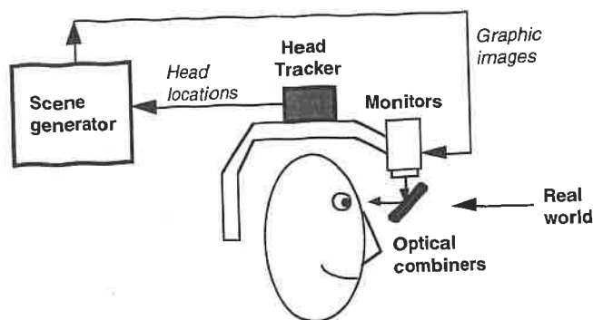
Figure 11. Optical see-through HMD conceptual diagram.
