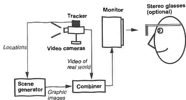
Figure 15. Monitor-based AR conceptual diagram.
