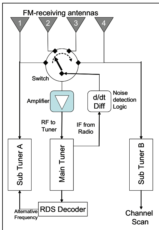
Fig. 13. Principle of switched diversity in modern tuners
