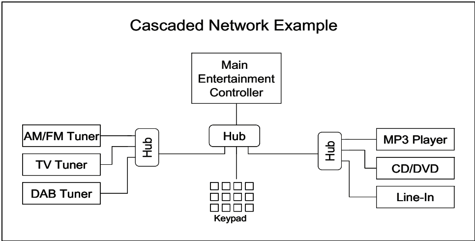
Fig. 4. Entertainment system organized in cascaded network architecture.
