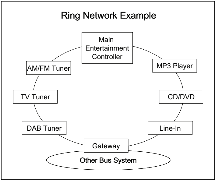
Fig. 3. Entertainment system organized in ring architecture
