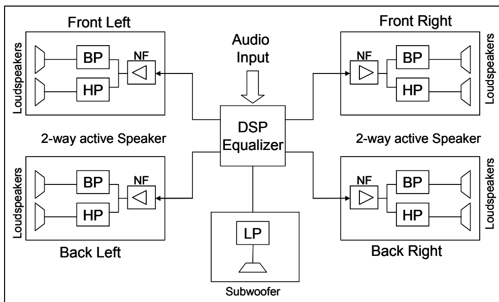
Fig. 14. Block diagram of modern sound system
