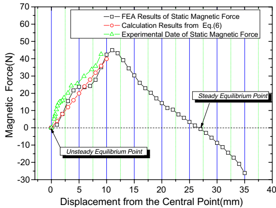
Fig. 6. Magnetic force without exciting current with displacement of the shuttle.
