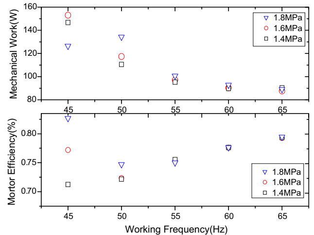
Fig. 14. Measured motor efficiency and mechanical work vs. working frequency at the input voltage of 15 V and different charging pressures.
