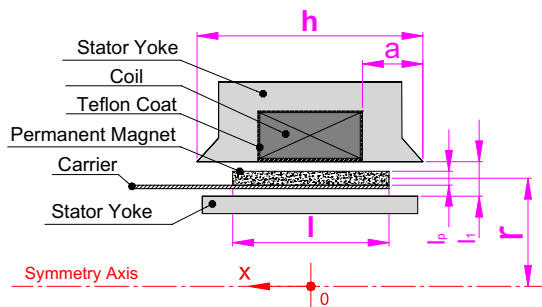
Fig. 1. Definitions of the geometrical dimensions of the moving magnet linear motor.
