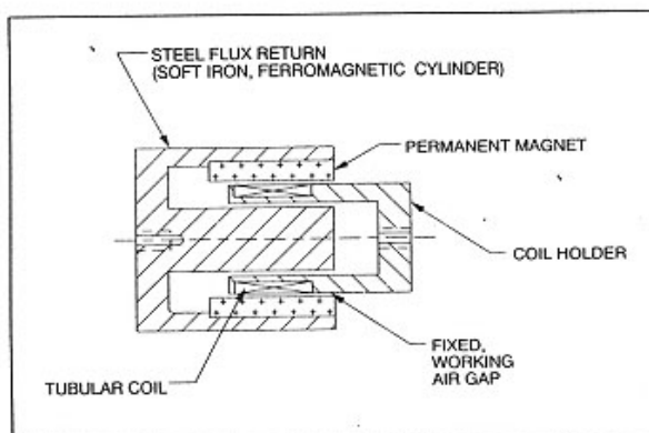
Figure 2. Linear Voice Coil Actuator.
