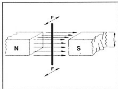
Figure 1. Lorentz Force Principle.
