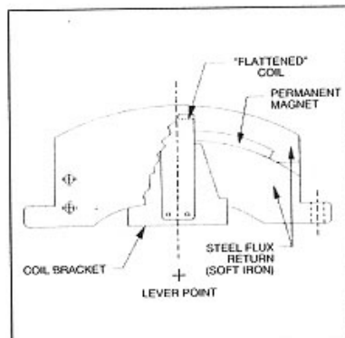
Figure 3. Rotary Voice Coil Actuator.
