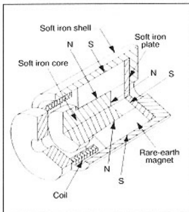
Figure 5. Flux-Focus Voice Coil Actuator Configuration.
