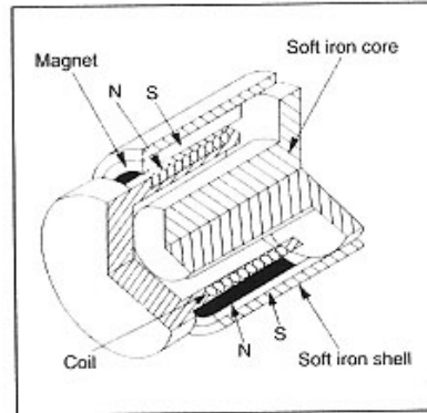
Figure 4. Conventional Voice Coil Actuator Configuration.
