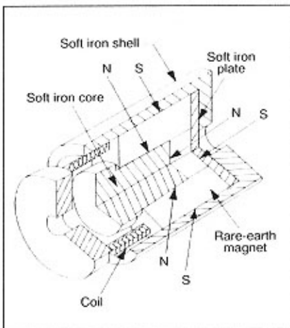
Figure 5. Flux-Focus Voice Coil Actuator Configuration.
