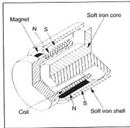
Figure 4. Conventional Voice Coil Actuator Configuration.
