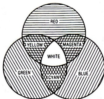
Chrominance primaries.
