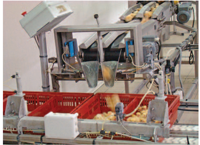
Chick counting machine.
