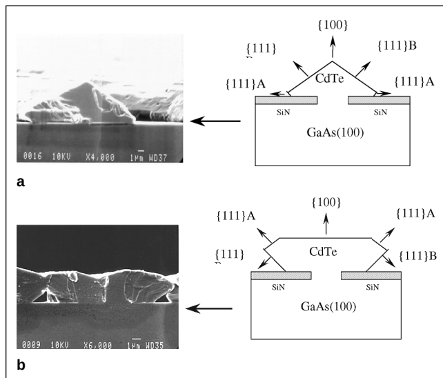
Fig. 6. SEM and corresponding schematic cross section of CdTe grown on GaAs (100) substrate at 550°C. (a) Growth window aligned to the [011] direction, 3 μm wide window with 20 μm spacing, (b) Growth window aligned to the [011] direction, 5 μm wide window with 6 μm spacing.
