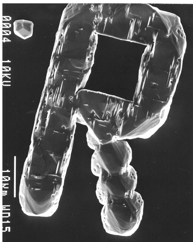
Fig. 4. Selective growth of CdTe on GaAs (100) using \text{SiN}_x as the mask. The letter R shows the importance of aligning the edges of openings to one of the major axis.
