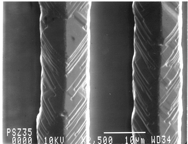
Fig. 7. Selective growth of CdTe on CdTe (211)B/Si substrate in the window stripe oriented along [011] direction at 550°C. The width and spacing of growth windows are 3 μm and 20 μm, respectively.
