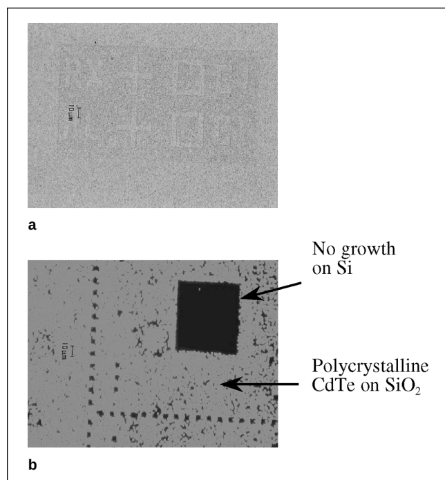
Fig. 1. Selective growth of CdTe on Si substrate with different mask layers. (a) Growth of CdTe on both Si and SiO 2 when T < 450^\circ\text{C} and P > 50 torr, (b) Polycrystalline CdTe growth on masked SiO 2 region, but no growth on Si surface when T > 450^\circ\text{C} and P < 50 torr.
