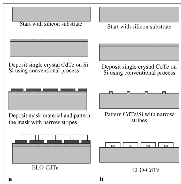
Fig. 2. Schematic diagram of process steps to get high quality ELO-CdTe on silicon substrate. (a) A conventional process, (b) an alternative process.
