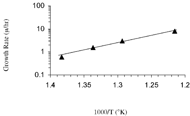
Fig. 5. Vertical growth rate as a function of temperature for CdTe films grown on patterned CdTe (211)B/Si substrate.
