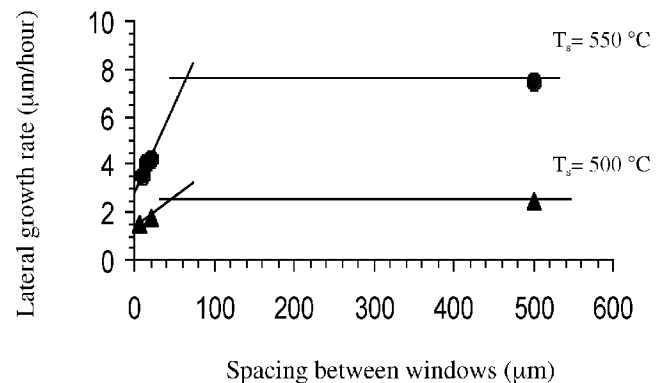
Fig. 8. Lateral growth rate as a function of the spacing between mask opening for two different growth temperatures.
