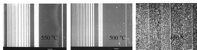
Fig. 3. Selectivity of the growth of CdTe at different temperatures on (a) GaAs(100) substrate with \text{SiN}_x mask layers, (b) CdTe (211)B/Si substrate with \text{SiN}_x mask layers.
