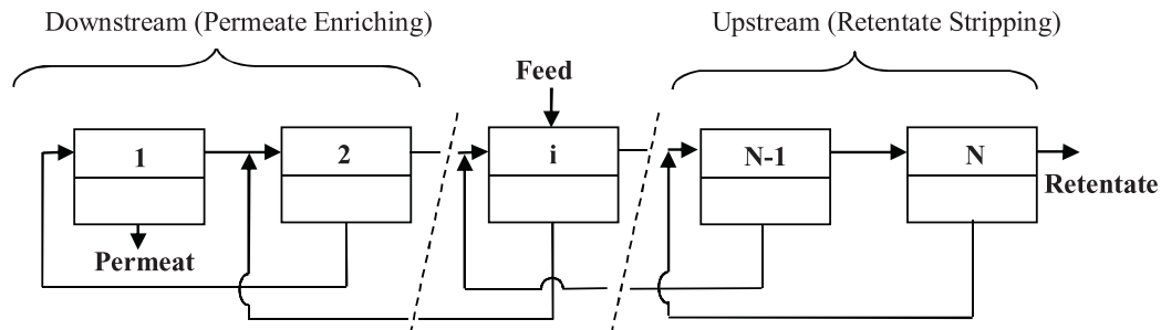
Fig. 1 Schematic of cascade membrane system with recycle.
