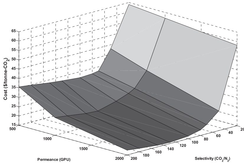
Fig.4 Dependence of objective function on membranes' selectivity and permeance.
