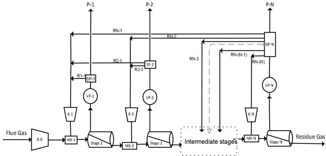
Fig. 3 Membrane superstructure network for optimization.
