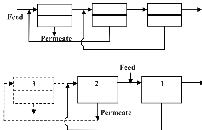
Fig. 2 Schematic of a) three-stage stripping b) two/three-stage enriching systems.
