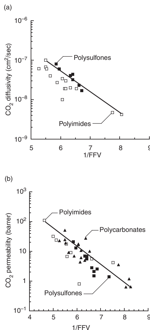
Figure 1.8 Correlations of (a) \text{CO}_2 diffusion and (b) \text{CO}_2 permeability coefficients with fractional free volume in glassy aromatic polysulfones, polyimides and polycarbonates. The experiments were conducted at 35^\circ\text{C} , a feed pressure of 10 atm while the permeate pressure was 'at vacuum' [76]
