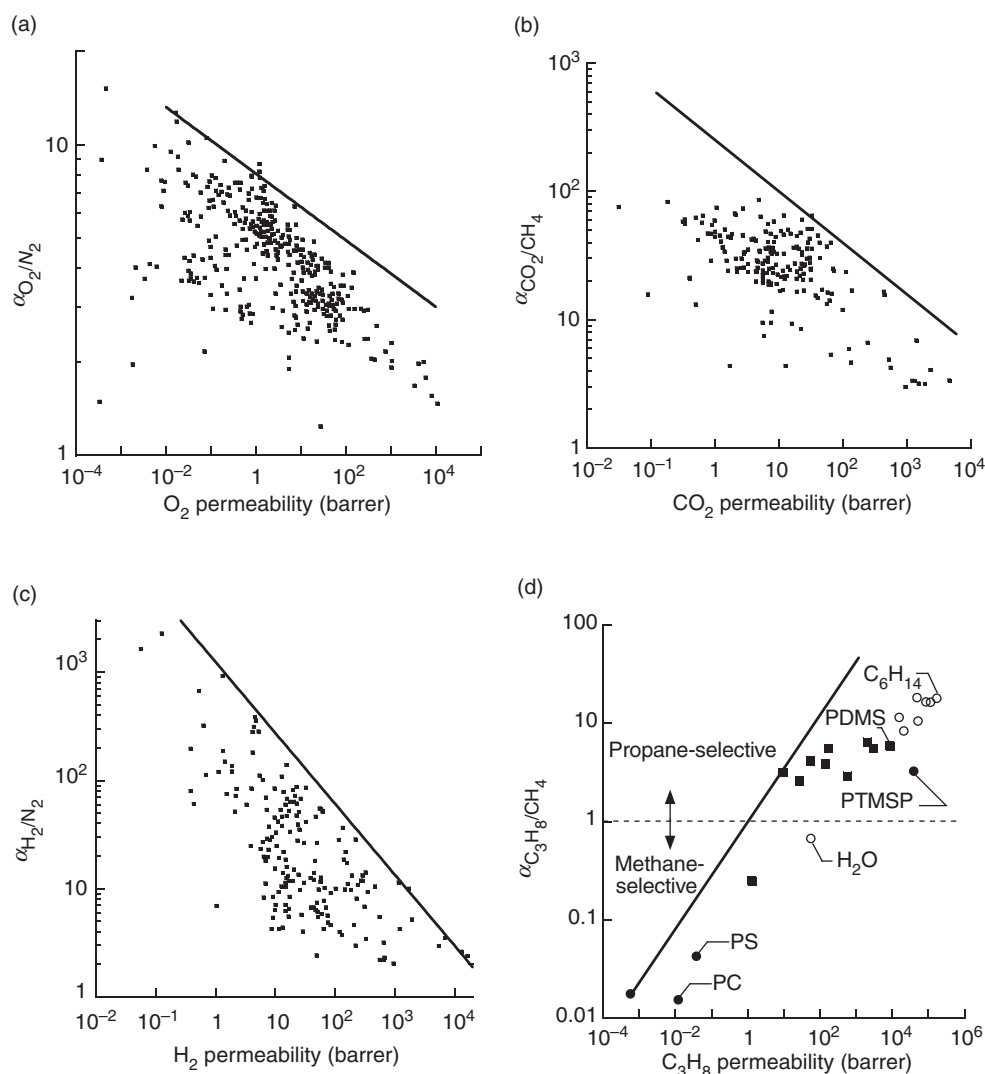
Figure 1.2 Permeability/selectivity trade-off maps for: (a) \text{O}_2/\text{N}_2 ; (b) \text{CO}_2/\text{CH}_4 ; (c) \text{H}_2/\text{N}_2 ; (d) \text{C}_3\text{H}_8/\text{CH}_4 [28]. For \text{O}_2/\text{N}_2 , \text{CO}_2/\text{CH}_4 and \text{H}_2/\text{N}_2 , the upper bound line was estimated by using the model given in Freeman [21], while for \text{C}_3\text{H}_8/\text{CH}_4 , the upper bound line was drawn by eye. (a–c) Reprinted from Journal of Membrane Science , 62 , I. M. Robeson, ‘Correlation of separation factor versus permeability for polymeric membranes’, 165–185, Copyright (1991), with permission from Elsevier. (d) Reprinted from Trends in Polymer Science , 5 , B. D. Freeman and I. Pinnau, ‘Separation of gases using solubility-selective polymers’, 167–173, Copyright (1997), with permission from Elsevier
