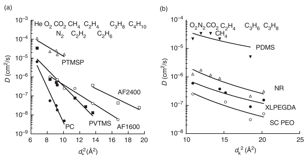
Figure 1.3 Dependence of diffusion coefficients on penetrant kinetic diameter in (a) glassy polymers at 23 °C, including poly(1-trimethylsilyl-1-propyne) (PTMSP), polyvinyltrimethylsilane (PVTMS), polycarbonate (PC), perfluorocarbon copolymers of 2,2-bis(trifluoromethyl)-4,5-difluoro-1,3-dioxole (BDD) and tetrafluoroethylene (TFE) containing 65 mol% BDD (AF1600) and 87 mol% BDD (AF2400) [39], and (b) rubbery polymers including cross-linked poly(ethylene glycol diacrylate) (XLPEGDA) at 35 °C [101], semicrystalline poly(ethylene oxide) (SC PEO) at 35 °C [32], natural rubber (NR) at 25 °C [33] and polydimethylsiloxane (PDMS) at 35 °C [34]. (a) Reprinted with permission from V. P. Shantarovich et al. , Macromolecules , 33 , 7453–7466 (2000). Copyright (2000) American Chemical Society. (b) (i) Reprinted from Journal of Membrane Science , 239 , H. Lin and B. D. Freeman, ‘Gas solubility, diffusivity and permeability in poly(ethylene oxide)’, 105–117, Copyright (2004), with permission from Elsevier; (ii) From ‘Flow of gases through polyethylene’, A. S. Michaels and H. J. Bixler, J. Polym. Sci. , 50 , 412–439, Copyright © 1961, John Wiley & Sons, Inc. Reprinted with permission of John Wiley & Sons, Inc.; (iii) From ‘Gas sorption, diffusion and permeation in polydimethylsiloxane’, T. C. Merkel, V. Bondar, K. Nagai, B. D. Freeman and I. Pinnau, J. Polym. Sci. Part B: Polym. Phys. Ed. , 38 , 415–434, Copyright © 2000, John Wiley & Sons, Inc. Reprinted with permission of John Wiley & Sons, Inc.; (iv) Reprinted with permission from H. Lin and B. D. Freeman, Macromolecules , 38 , 8394–8407 (2005). Copyright (2005) American Chemical Society
