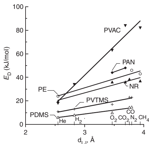
Figure 1.20 Effect of penetrant size on activation energy of diffusion in poly(vinyl acetate) (PVAC) (▼), polyacrylonitrile (PAN) (◆), polyethylene (PE) (○), natural rubber (NR) (▲), PVTMS (+) and PDMS (▲) [103]
