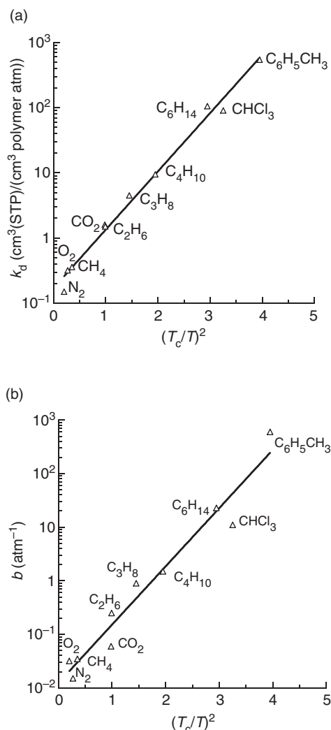
Figure 1.12 Correlation of (a) k_D and (b) b with squared reduced critical temperature in amorphous Teflon AF2400 [114]
