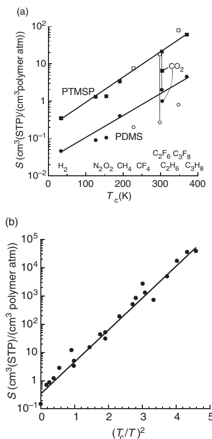
Figure 1.5 Correlation of low-pressure-limit solubility coefficients with solute critical temperature in (a) PTMSP and PDMS, and (b) AF2400 [12,88]. (a) From ‘Sorption and transport of hydrocarbon and perfluorocarbon gases in poly(1-trimethylsilyl-1-propyne)’, T. C. Merkel, V. Bondar, K. Nagai and B. D. Freeman, J. Polym. Sci. Part B: Polym. Phys. Ed. , 37 , 273–296, Copyright © 1999, John Wiley & Sons, Inc. Reprinted with permission of John Wiley & Sons, Inc. (b) (i) Reprinted with permission from V. Bondar et al. , Macromolecules , 32 , 6163–6171 (1999). Copyright (1999) American Chemical Society; (ii) Reprinted with permission from T. C. Merkel et al. , Macromolecules , 32 , 8427–8440 (1999). Copyright (1999) American Chemical Society
