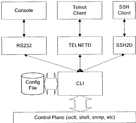
This diagram shows the high-level CLI interfaces.
