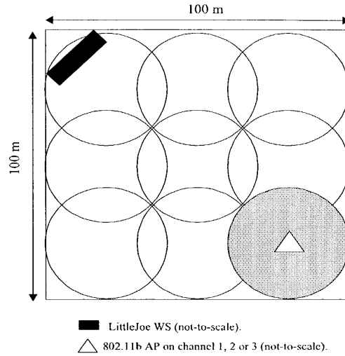
Figure 2 Reference LittleJoe indoor deployment.
