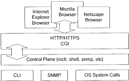
This diagram shows the high-level HTTP module interfaces.
