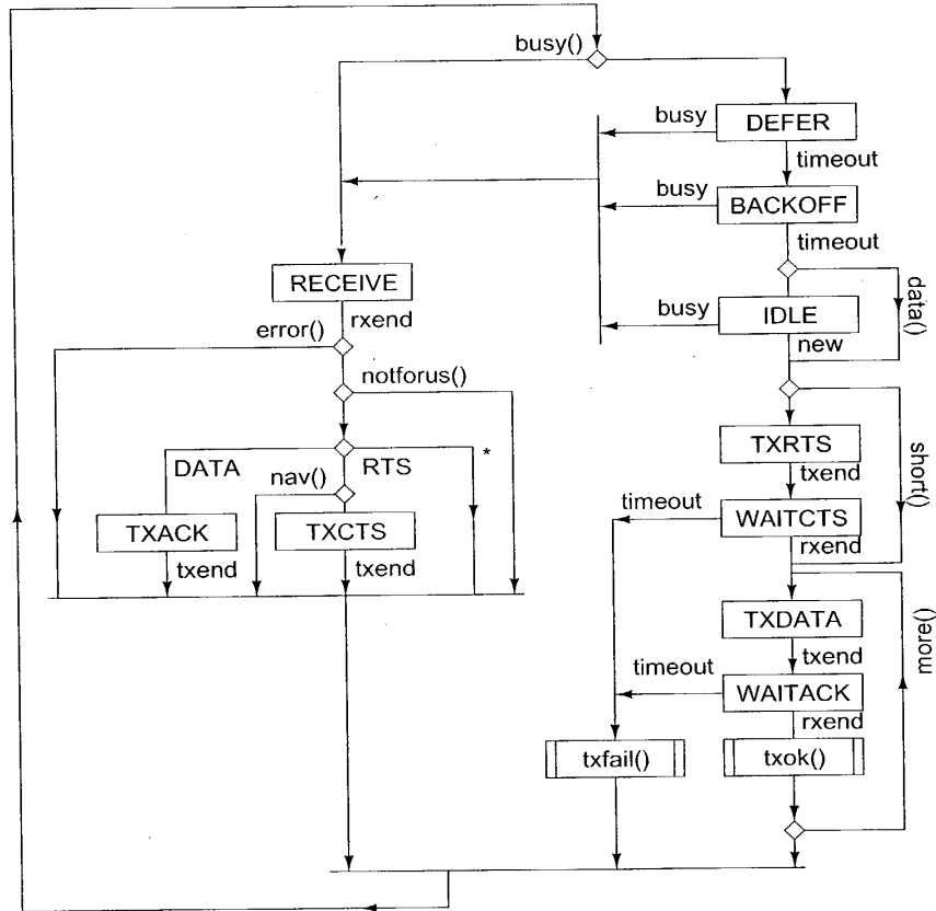
Figure 2: State transition diagram for the MAC controller.
