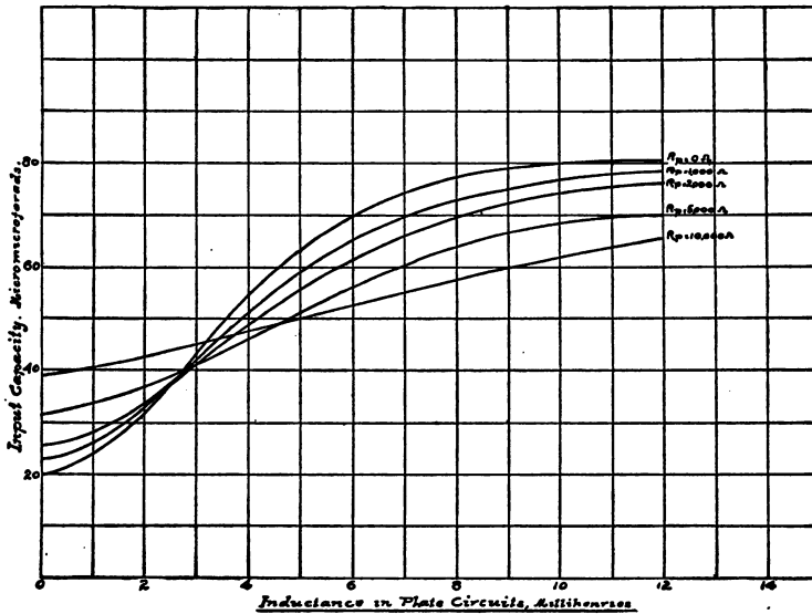
FIG. 7.—Variation in input capacity with inductive load
