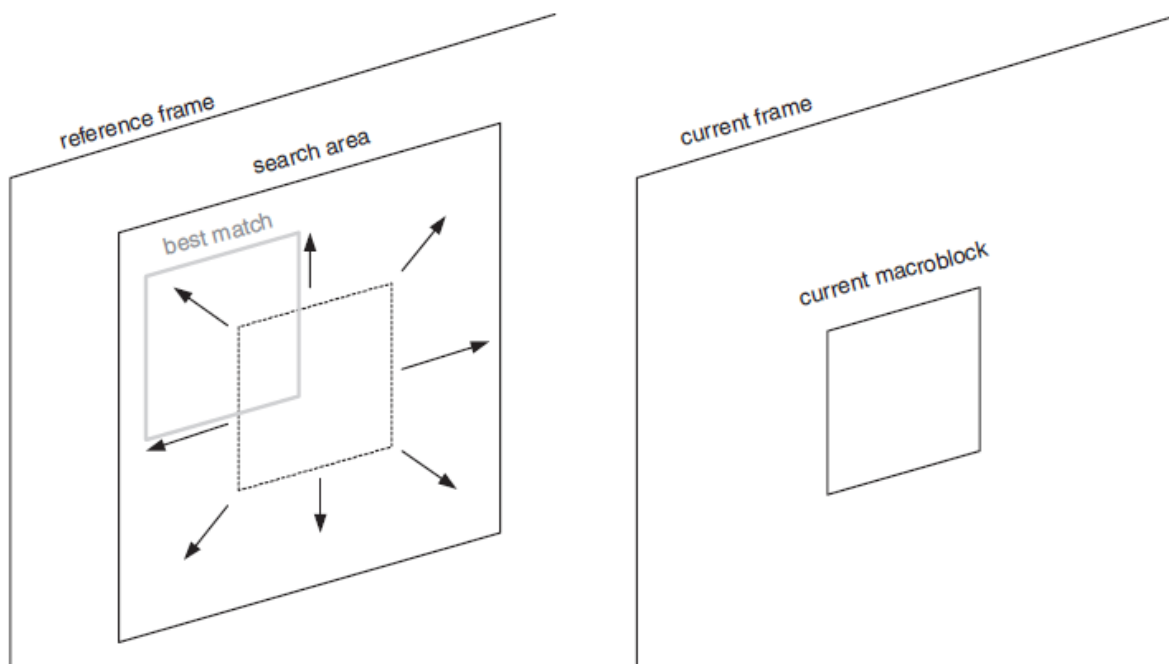
Figure 3.9 Motion estimation
