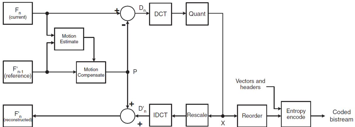
Figure 3.51 DPCM/DCT video encoder
