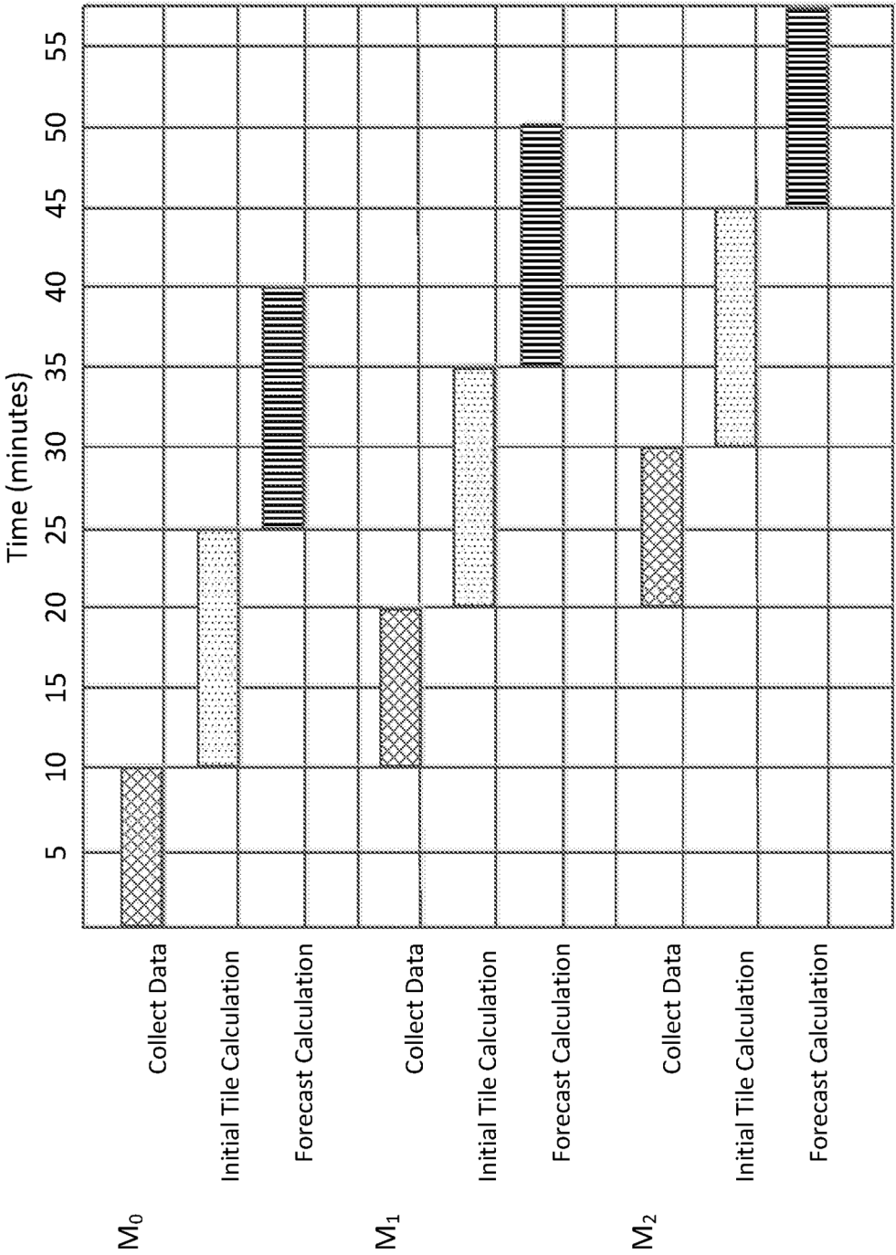
Cadence Process Timing FIGURE 4
