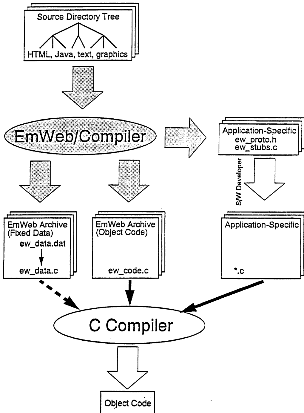
Figure 1: EmWeb/Compiler
