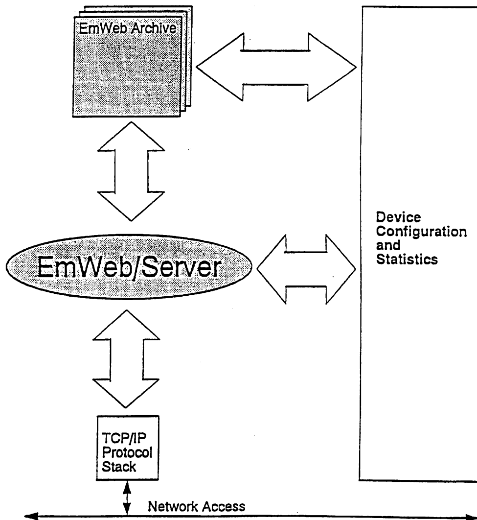
Figure 2: EmWeb/Server
