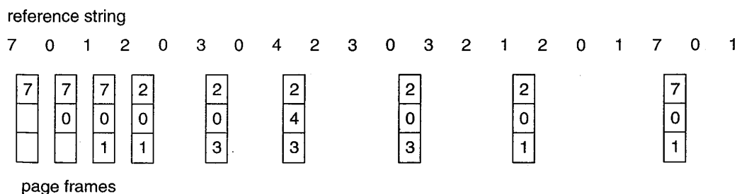
Figure 9.10 Optimal page-replacement algorithm.
