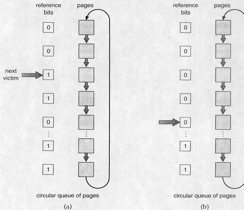
Figure 9.13 Second-chance (clock) page-replacement algorithm.
