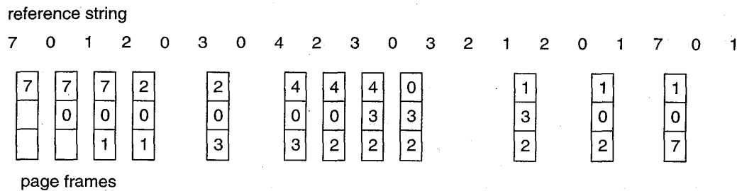
Figure 9.11 LRU page-replacement algorithm.
