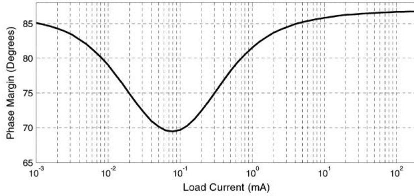
Fig. 7. Phase margin of the proposed LDO loop-gain transfer function under different load currents with a 1- \mu F output capacitor.
