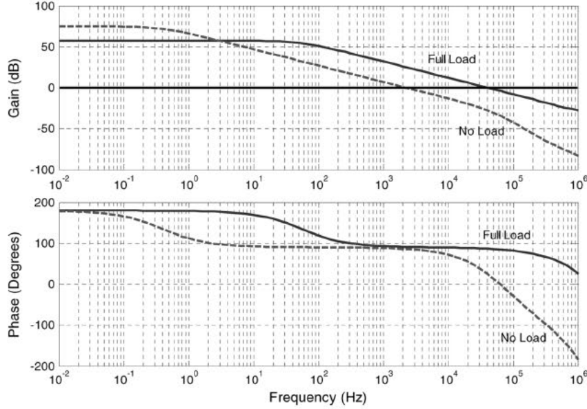
Fig. 6. Simulated loop-gain transfer function of the proposed LDO with a 1 \mu F output capacitor.
