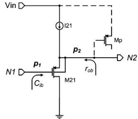
Fig. 2. Source-follower implementation of the intermediate buffer stage.
