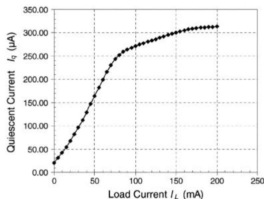
Fig. 10. Measured quiescent current under different load currents.
