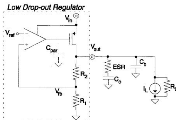
Fig. 1. Typical low drop-out regulator topology.
