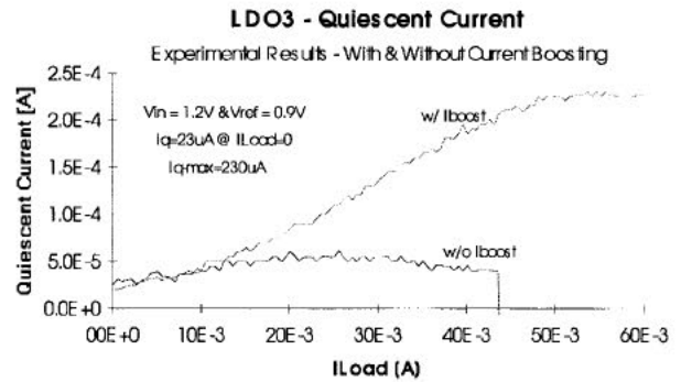
Fig. 11. Quiescent current as a function of load-current.
