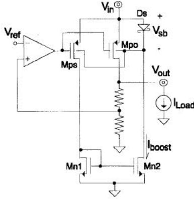
Fig. 6. LDO with current boosting capabilities.
