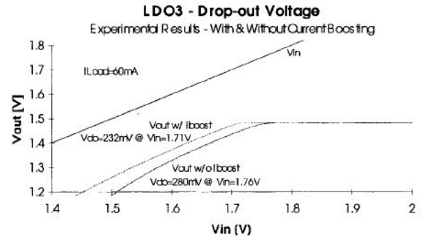
Fig. 12. Drop-out voltage performance at 60 mA of load-current.
