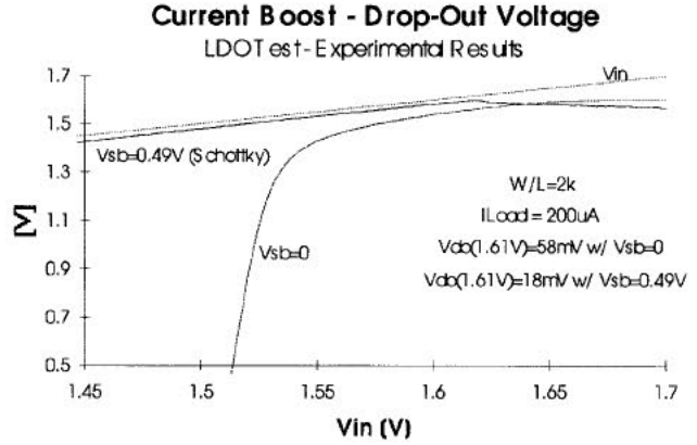
Fig. 7. Drop-out voltage performance of the current boost topology.
