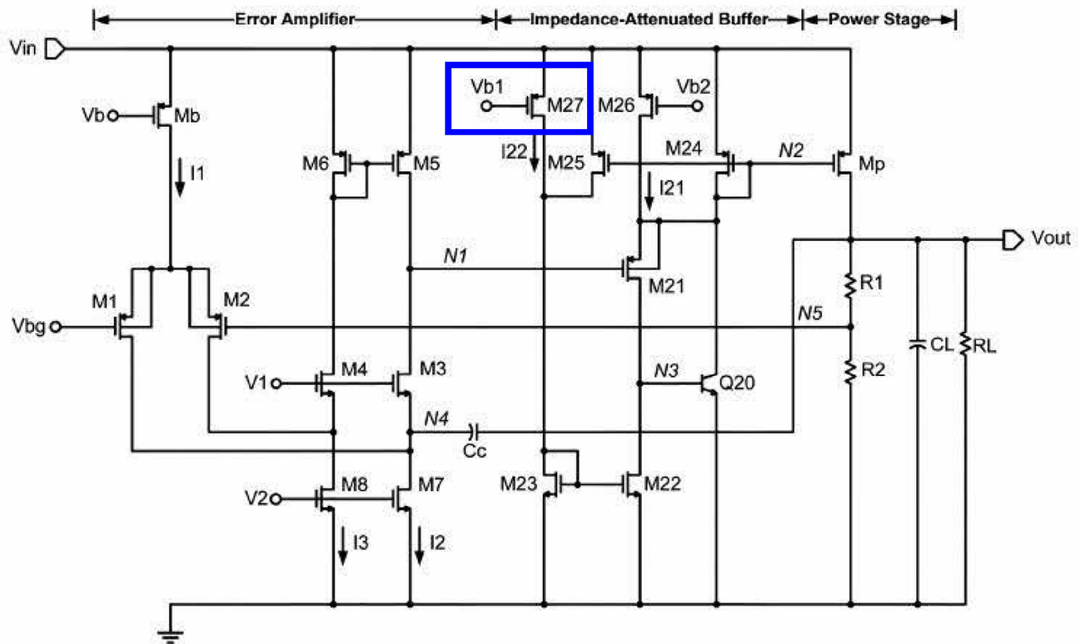
Fig. 8. Schematic of the proposed LDO.
