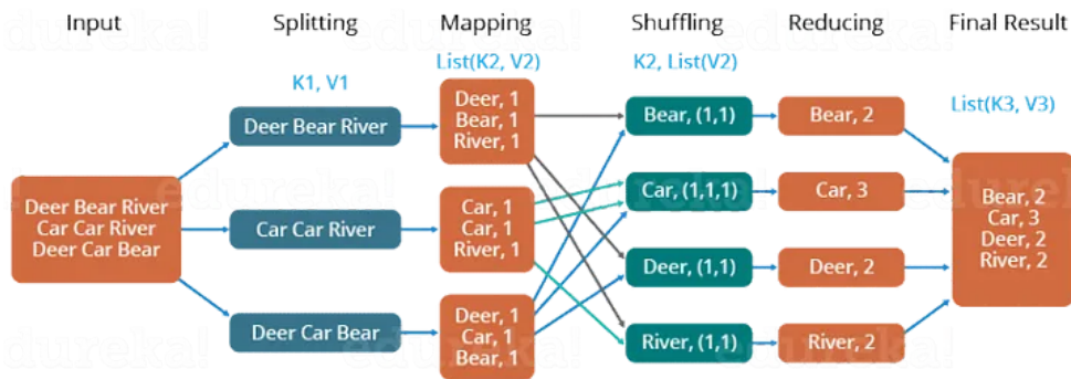
MapReduce Example - MapReduce Tutorial
