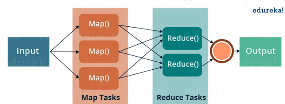
What is MapReduce - MapReduce Tutorial
