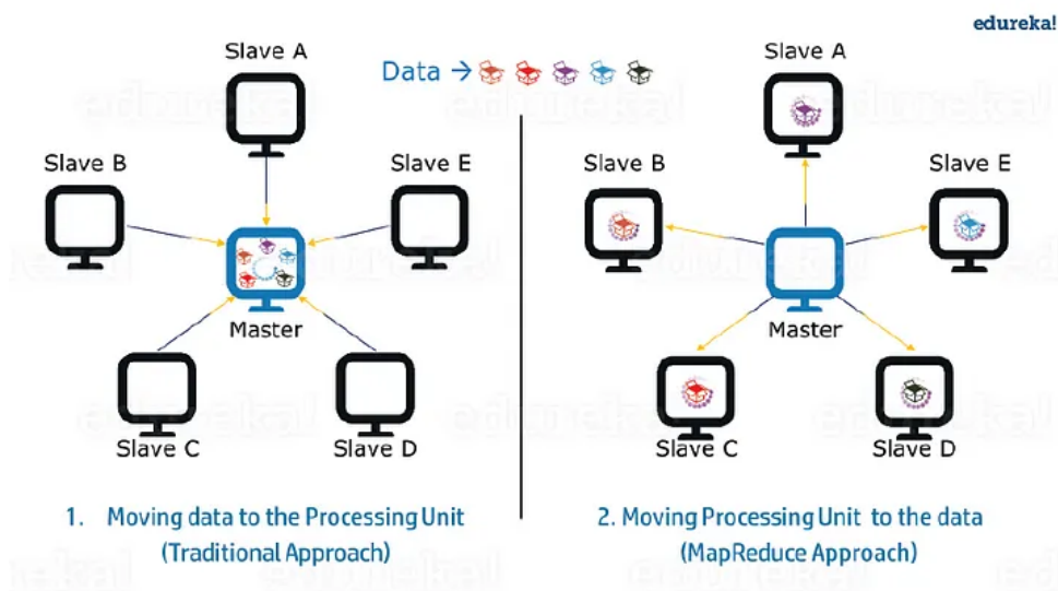
Traditional Way Vs. MapReduce Way - MapReduce Tutorial
