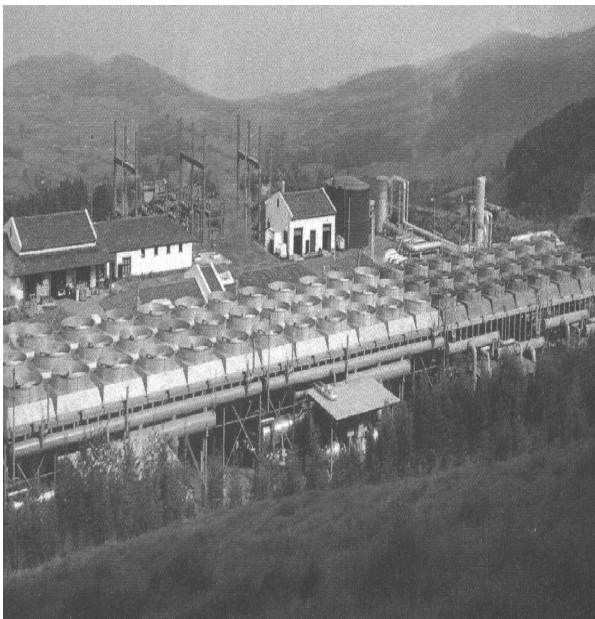
Figure 6. São Miguel 14 MW Air Cooled Binary Two Phase Geothermal Plant
