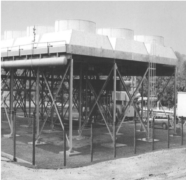
Figure 5. Kawerau 3.8 MW Air Cooled Binary Geothermal Plant
