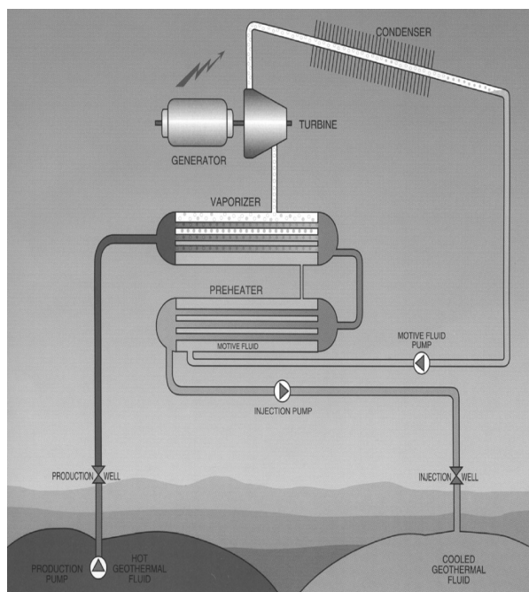
Figure 1. Process Diagram: Air Cooled Binary Geothermal Power Plant
