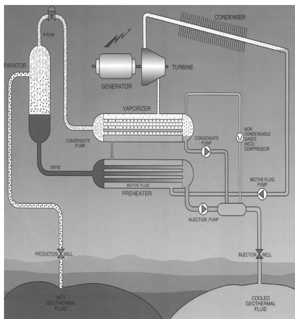
Figure 2. Process Diagram: Two-Phase Binary Geothermal Power Plant
