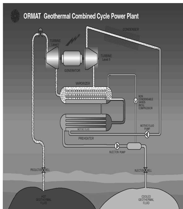
Figure 3. Process Diagram: ORMAT® Combined Cycle Unit
