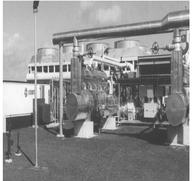
Figure 7. Rotokawa 27 MW Air Cooled Geothermal Combined Cycle Plant
