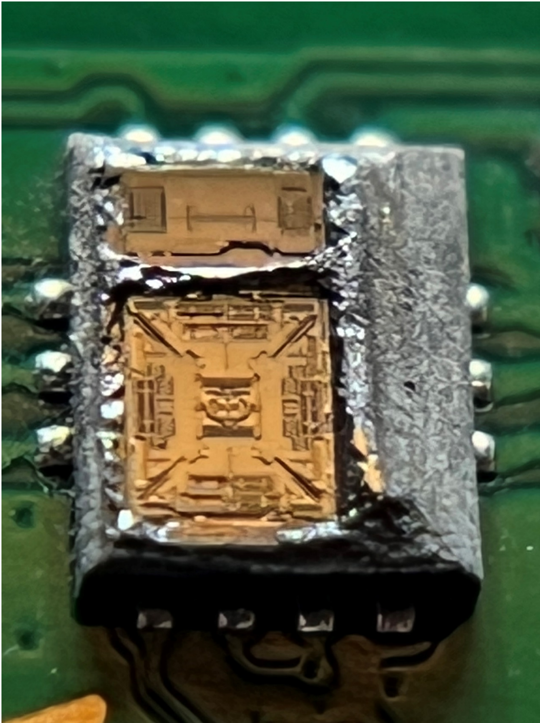
Image of MEMS accelerometer (top portion) and 3-axis MEMS gyroscope (bottom) in disassembled STMicroelectronics IMU chip found in Nintendo Switch product
