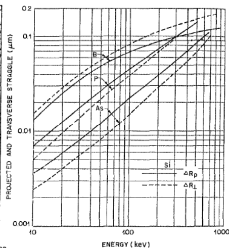
Fig. 10-8 Calculated ion projected straggle \Delta R_p , and ion lateral straggle \Delta R_t for As, P, and B ions in silicon. After Smith, Ref. 7, redrawn by Seidel in Ref. 83, Copyright, 1983, Lucent Technologies, Incorporated. Reprinted by permission.
