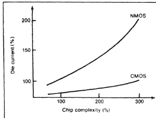
Fig. 16-3 As circuit complexity increases, NMOS power consumption rises to levels that eventually prevent further growth. In contrast, CMOS power consumption increases only slightly as the device count on a chip rises.
