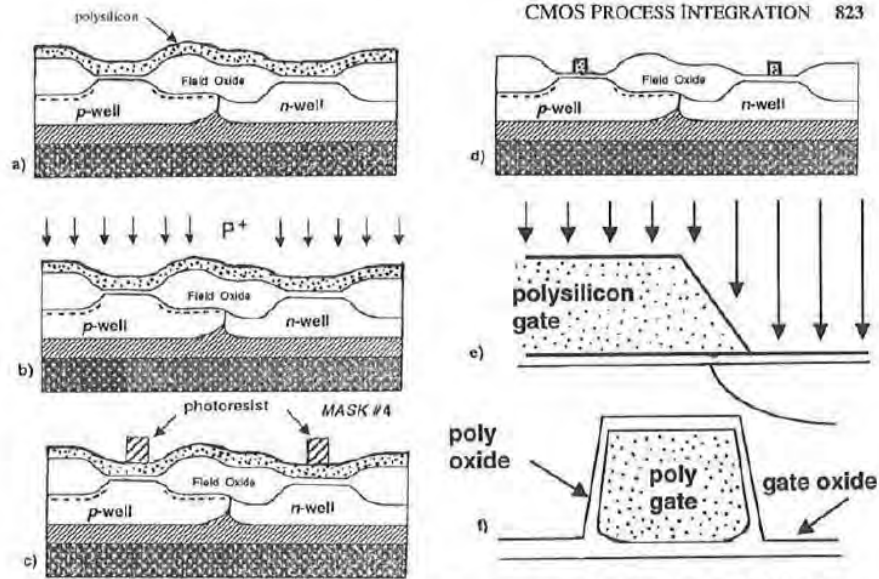
Fig. 16-14 n^+ -polysilicon gate formation: (a) deposition of undoped polysilicon film by LPCVD; (b) ex-situ doping of the polysilicon with phosphorus by chemical diffusion of ion implantation; (c) Use Mask #4 to define the polysilicon gates; (d) etch polysilicon and strip resist; (e) the etch process used to pattern the gate must yield poly features with vertical sidewalls (to maintain control of the effective gate length during the implant process that forms the source and drain regions); (f) polysilicon re-ox step grows a thin oxide on the poly by a short thermal oxidation process.
