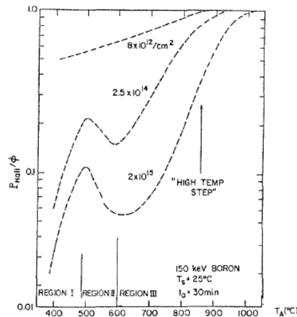
Fig. 10-20 Isochronal annealing behavior of boron. The ratio of free-carrier content, p_{\text{Hall}} , to dose \phi is plotted against anneal temperature T_A for three doses of boron. 32 Reprinted with permission of Gordon and Breach Publishing Company.
