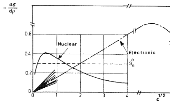
Fig. 10-6 (a) Nuclear stopping power for Thomas-Fermi potential (solid line) and electronic stopping power (dash-dot line) for k = 0.15 in terms of the reduced variables \varepsilon and \rho , based on LSS theory. 3
