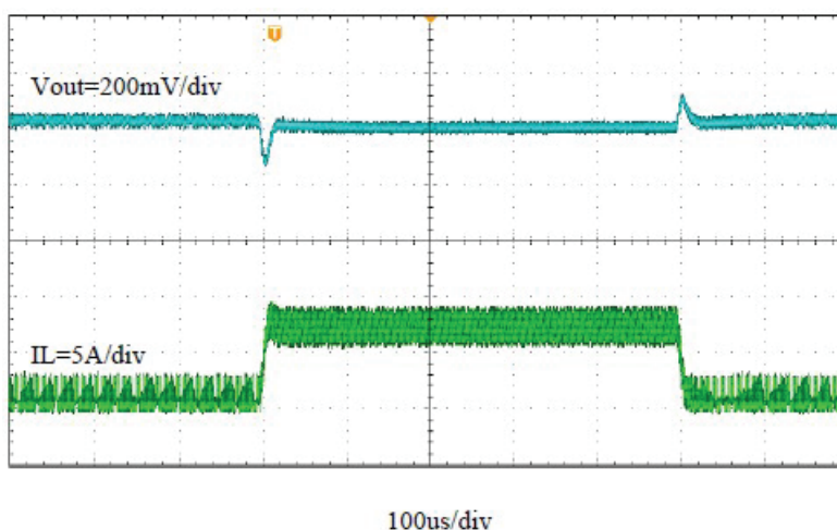
Figure 4-1. TPS51395 Transient Waveform
