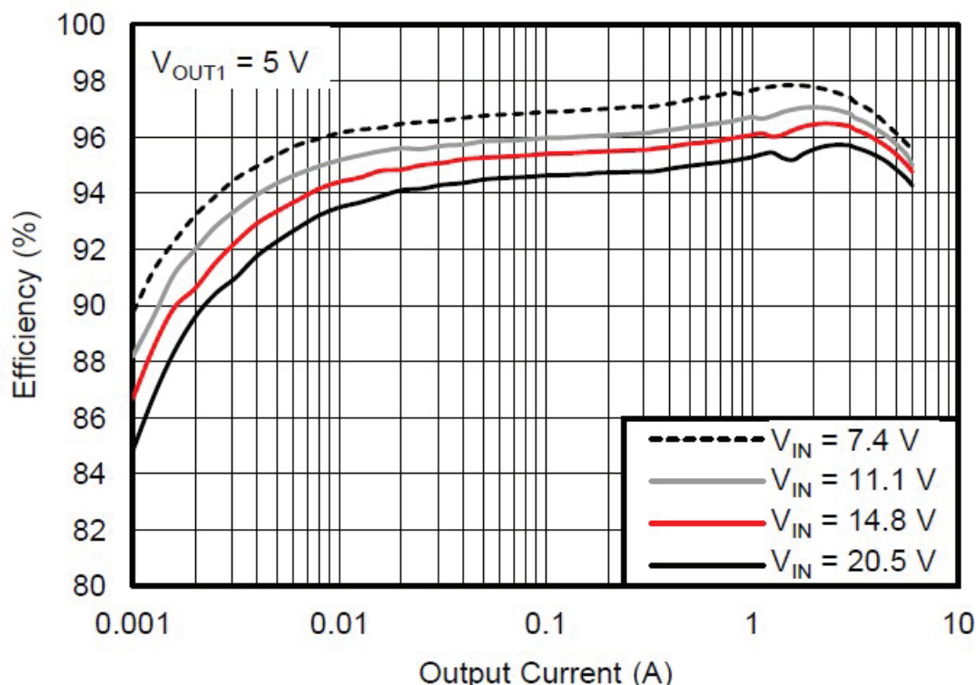
Figure 2-1. TPS51825A Efficiency Plot
