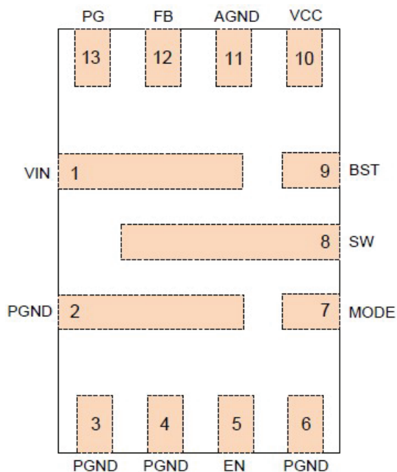
Figure 5-1. TPS566335 in 2x3mm QFN Package
