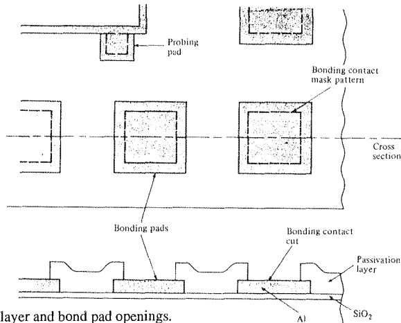
Fig. 16-20 Passivation layer and bond pad openings.
