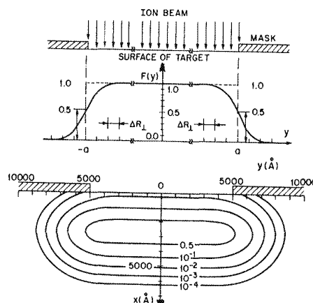
Fig. 10-3 Illustration of lateral profiles. (a) Ion concentration along the lateral direction ( y ) for a gate mask with a \gg \Delta R_{\perp} and infinite extension in the x -direction. (b) Contours of equal-ion concentrations for 70 keV B^+ ( R_p = 2710 Å, \Delta R_p = 824 Å, and \Delta R_{\perp} = 1006 Å) incident into silicon through a 1 \mu\text{m} slit. 6 Reprinted with permission of the Japanese Journal of Applied Physics.
