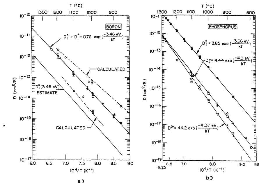
Fig. 9-7 Intrinsic diffusion coefficients vs. temperature for: a) boron; b) phosphorus. 13 Reprinted with permission of North Holland Publishing Co.
