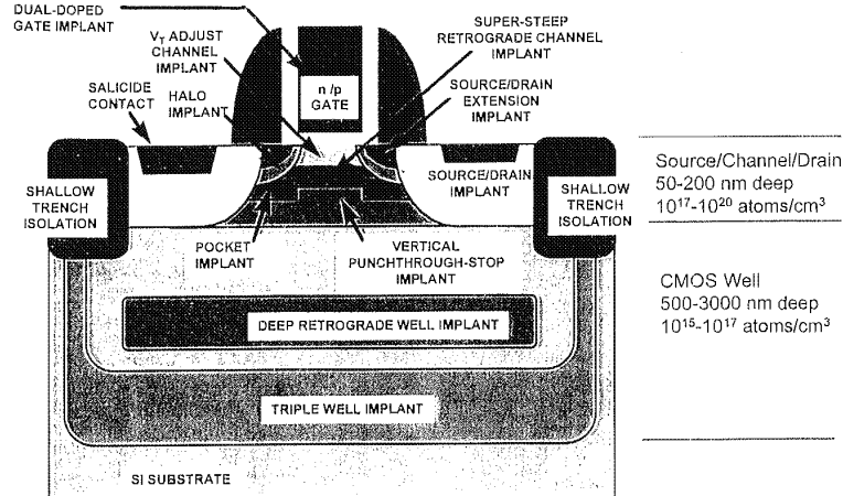
Fig. 10-40 CMOS transistor doping regions.
