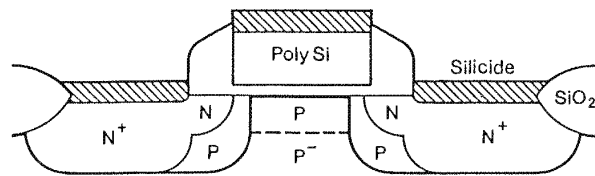
Figure 1. DI-LDD device cross section.
