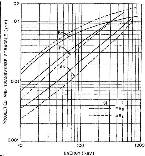
Fig. 10-8 Calculated ion projected straggle \Delta R_p , and ion lateral straggle \Delta R_L for As, P, and B ions in silicon. After Smith, Ref. 7, redrawn by Seidel in Ref. 83, Copyright, 1983, Lucent Technologies, Incorporated. Reprinted by permission.
