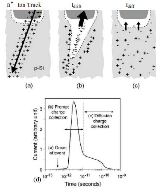
Fig. 2. Schematic representation of charge collection in a silicon junction immediately after (a) an ion strike, (b) prompt (drift) collection, (c) diffusion charge collection, (d) the junction current induced as a function of time [4].
