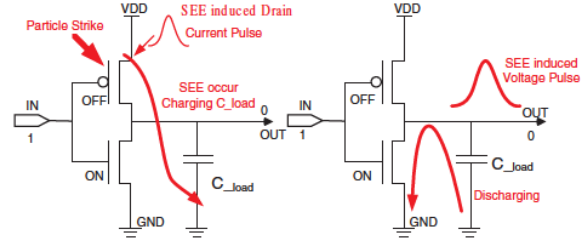
Fig. 3. An schematic view of how SEE-induced current pulse translates into a voltage pulse in a CMOS inverter.
