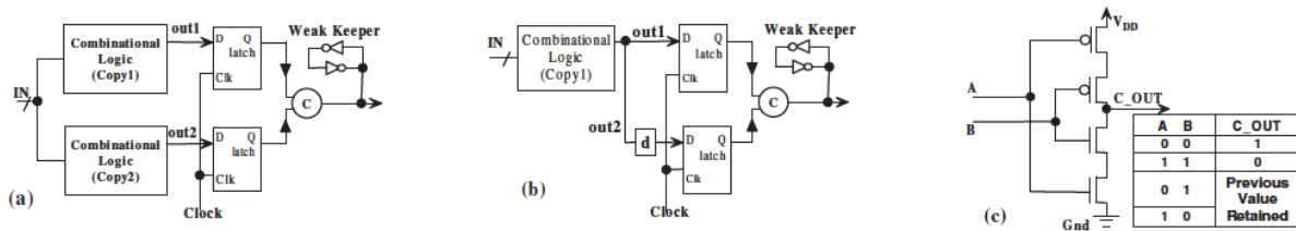
Fig. 4. Error correction using duplication, (a) space redundancy structure, (b) time redundancy structure, and (c) C-element [17].
