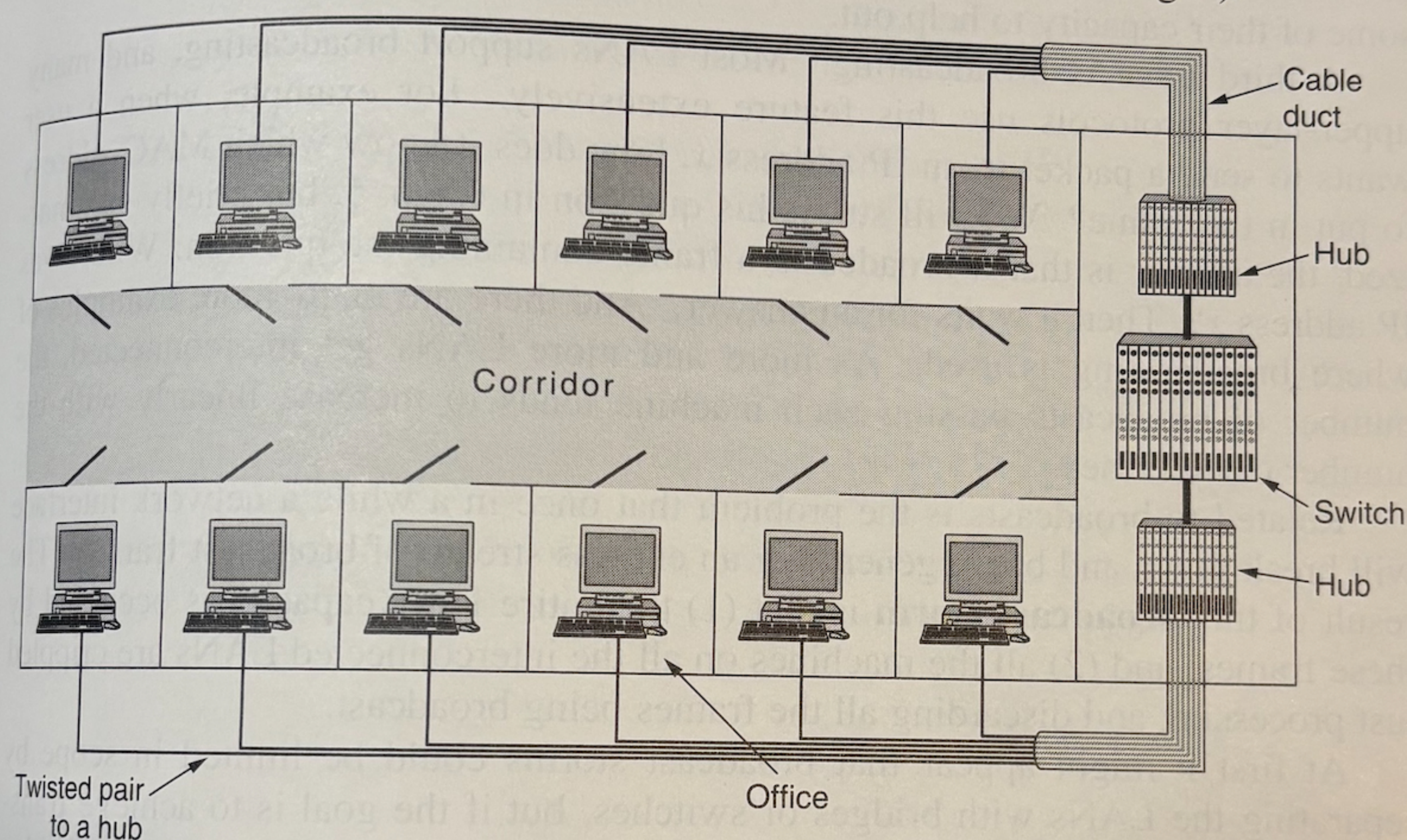
Figure 4-48. A building with centralized wiring using hubs and a switch.
