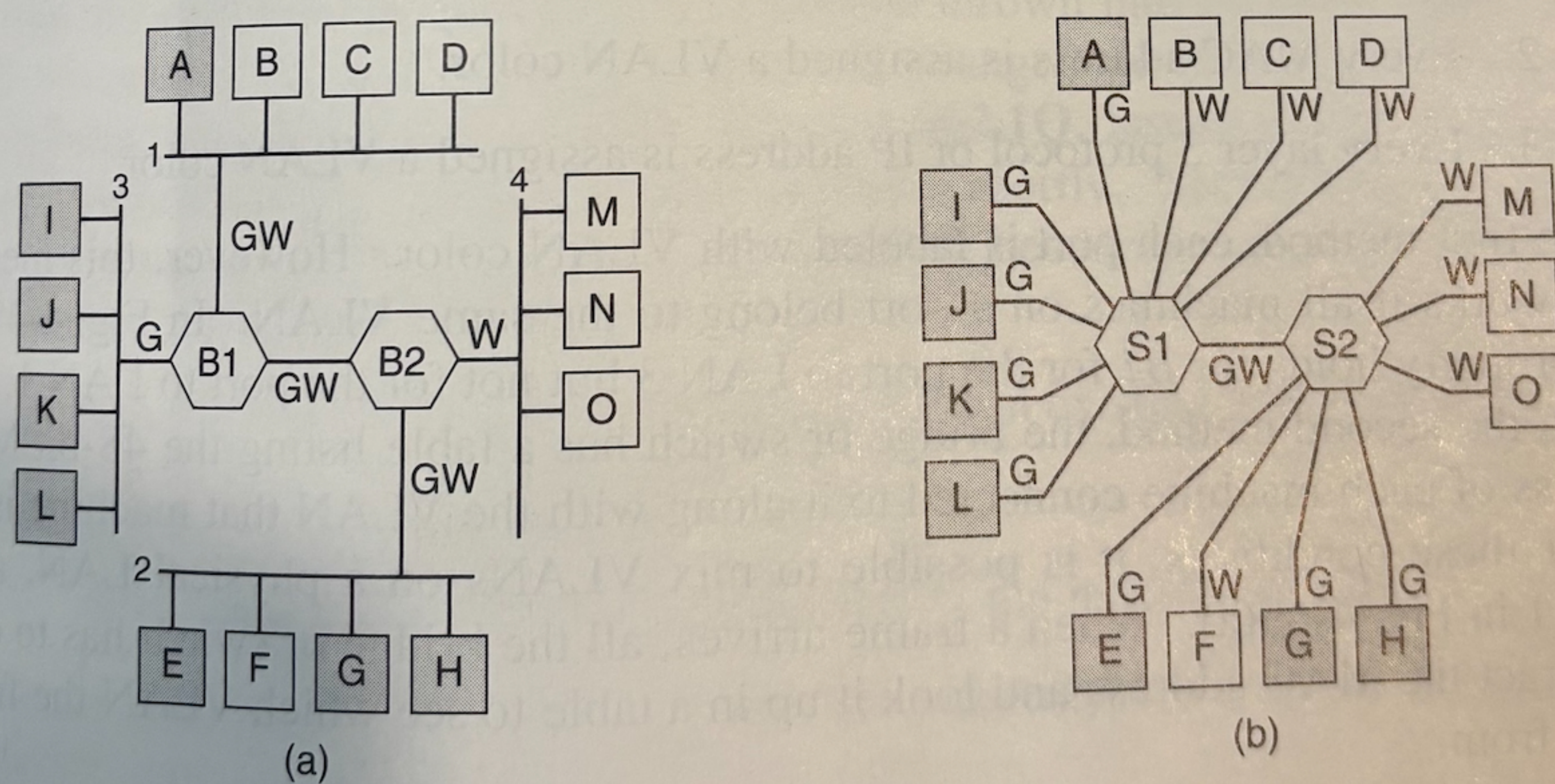
Figure 4-49. (a) Four physical LANs organized into two VLANs, gray and white, by two bridges. (b) The same 15 machines organized into two VLANs by switches.
