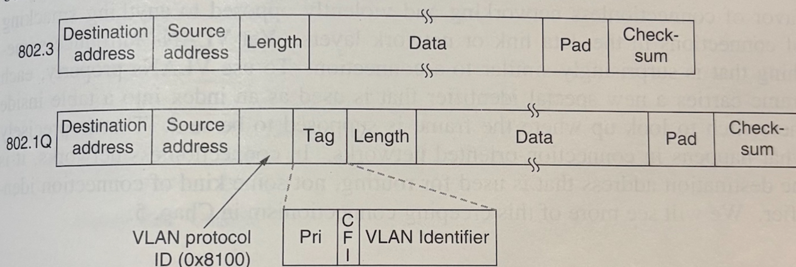
Figure 4-51. The 802.3 (legacy) and 802.1Q Ethernet frame formats.
