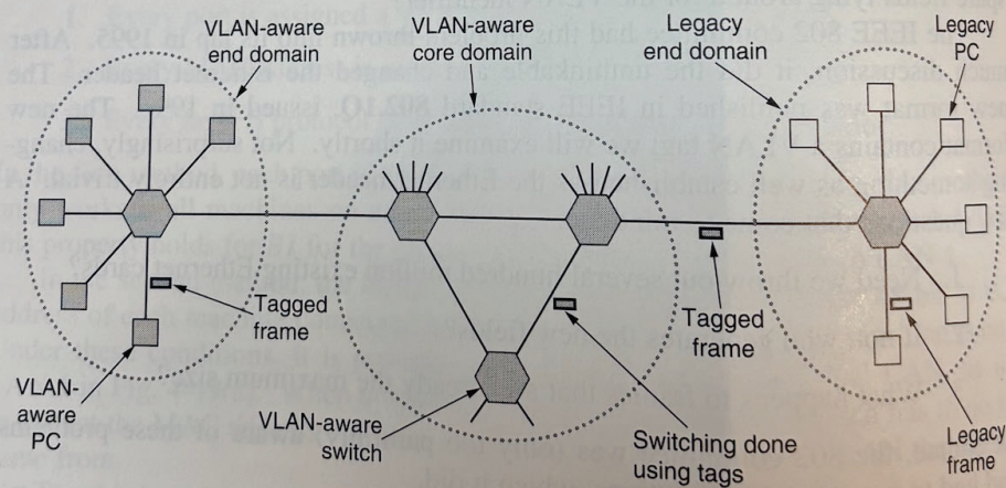
Figure 4-50. Transition from legacy Ethernet to VLAN-aware Ethernet. The shaded symbols are VLAN aware. The empty ones are not.
