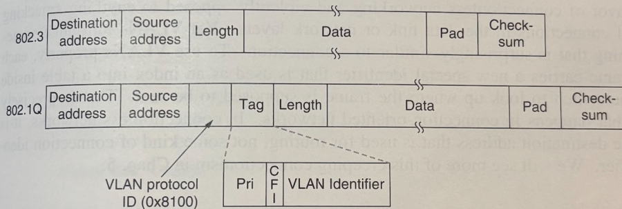
Figure 4-51. The 802.3 (legacy) and 802.1Q Ethernet frame formats.
