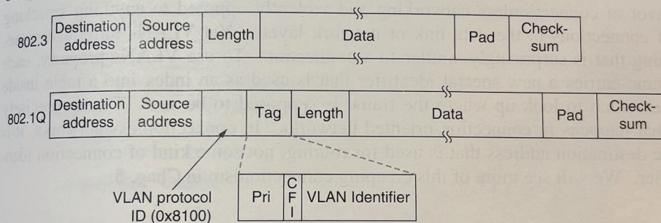
Figure 4-51. The 802.3 (legacy) and 802.1Q Ethernet frame formats.
