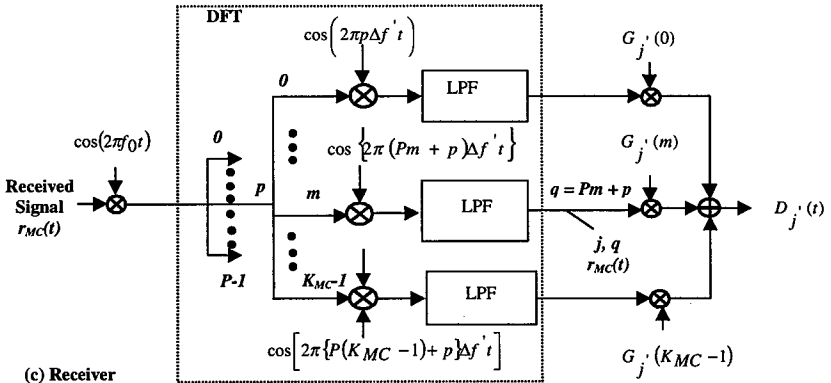
(c) Receiver
