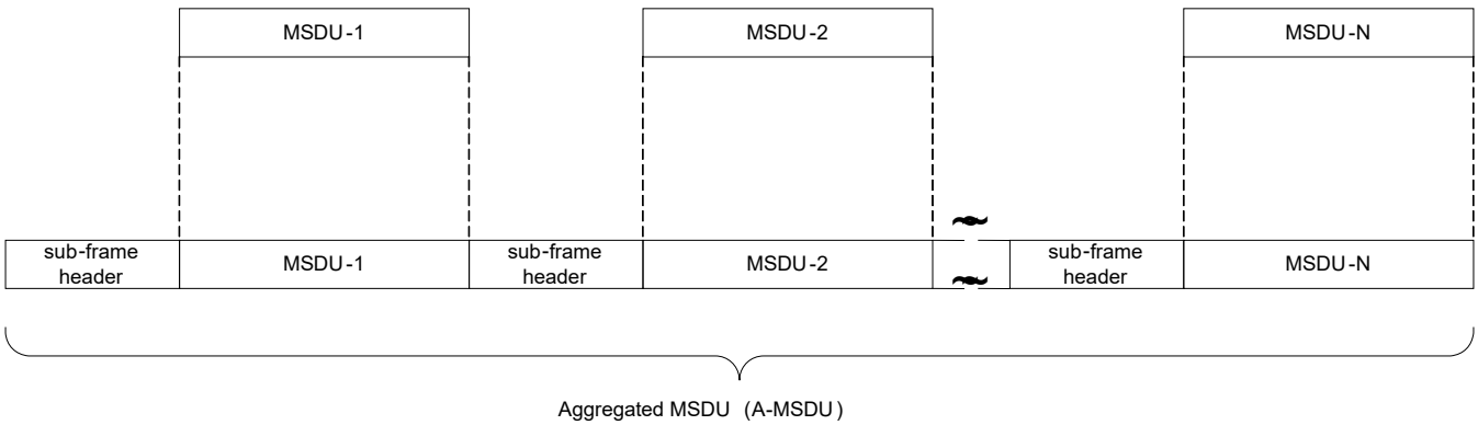
Figure 001n – Formation of an A-MSDU
