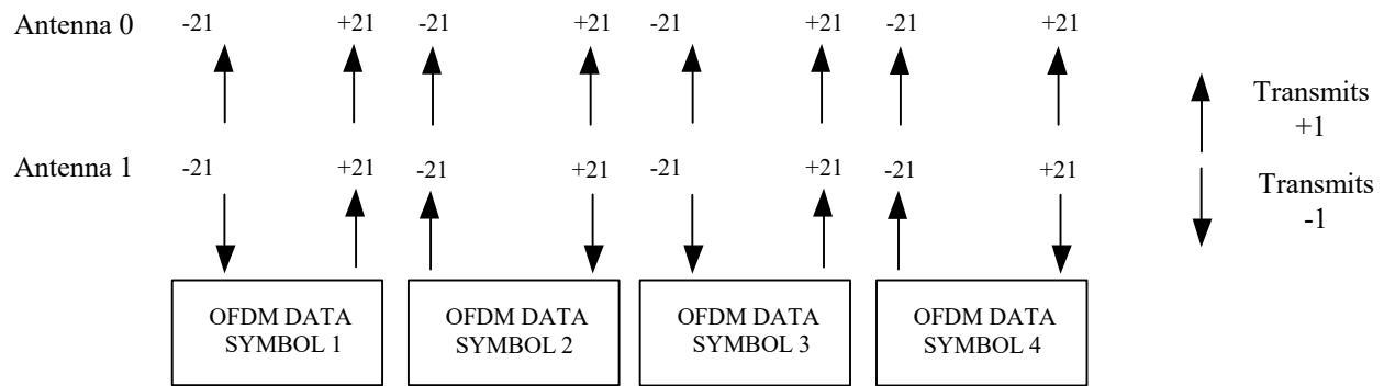
Figure 023 – An illustration of the relative polarity of pilot signals in the 2TX, 20 MHz mode. “-21” and “+21” indicate the subcarrier indexes on which pilot signals are sent
