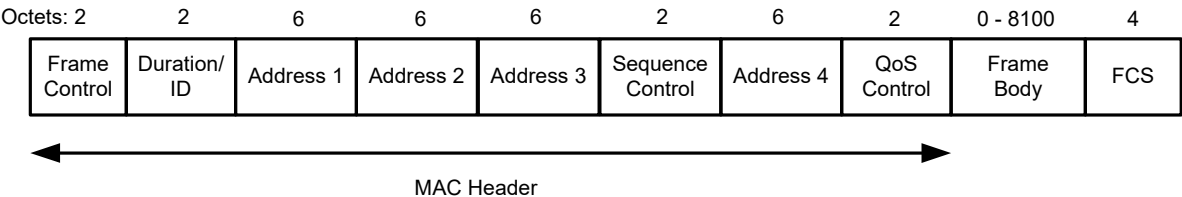
Figure 22 – Data frame
