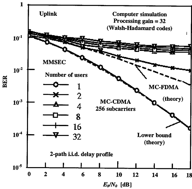
Figure 8.14 Uplink BER of MC-CDMA systems with MMSEC.
